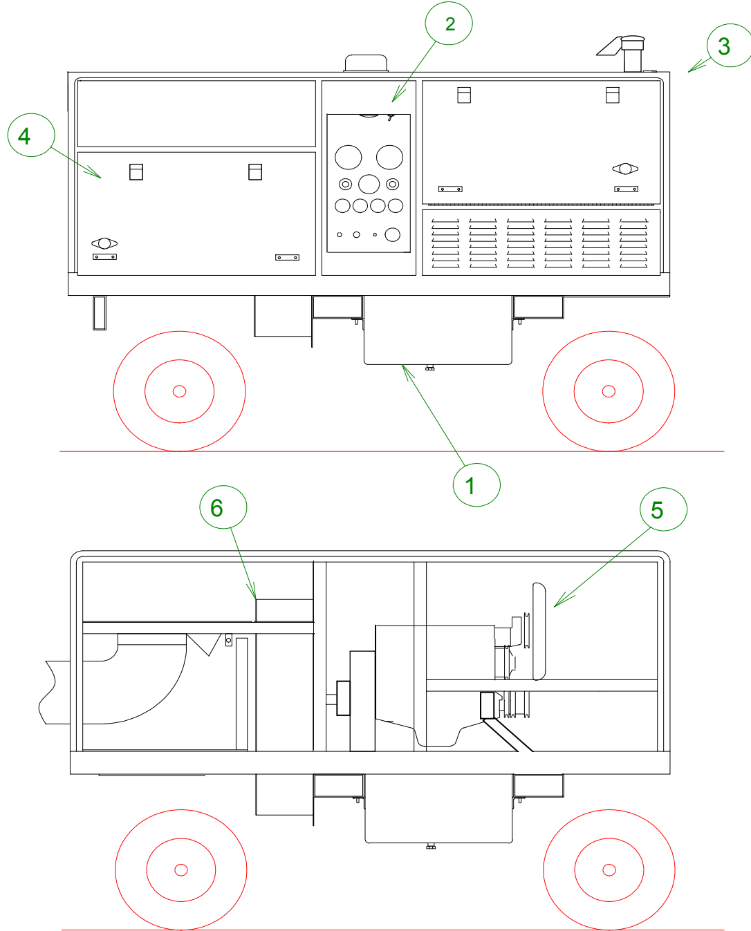
Figure 1. Final Assembly
