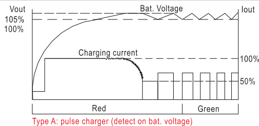
Type A: pulse charger (detect on bat. voltage)
