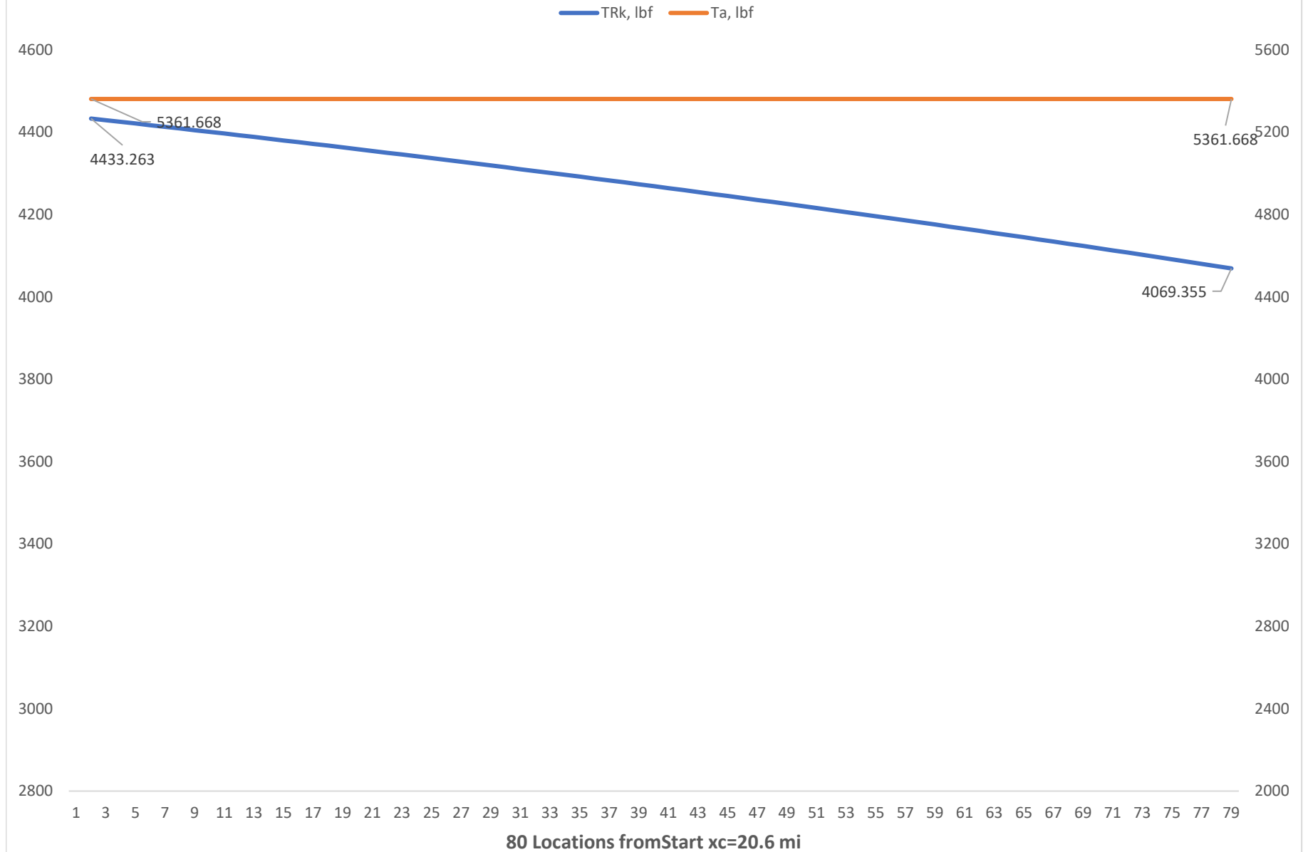
Executive Jet Cruising at 32000 ft: TRk (Thrust Req'd) vs. Ta (Thrust Available)
