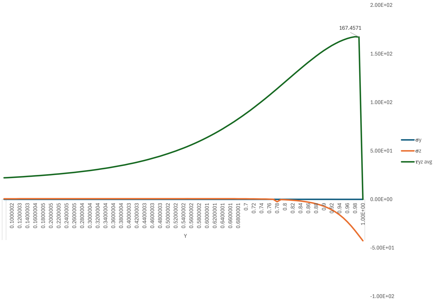
(90/0)s Laminate Interlaminar Stresse At Free Edge Region Y=1 and z=1/2
