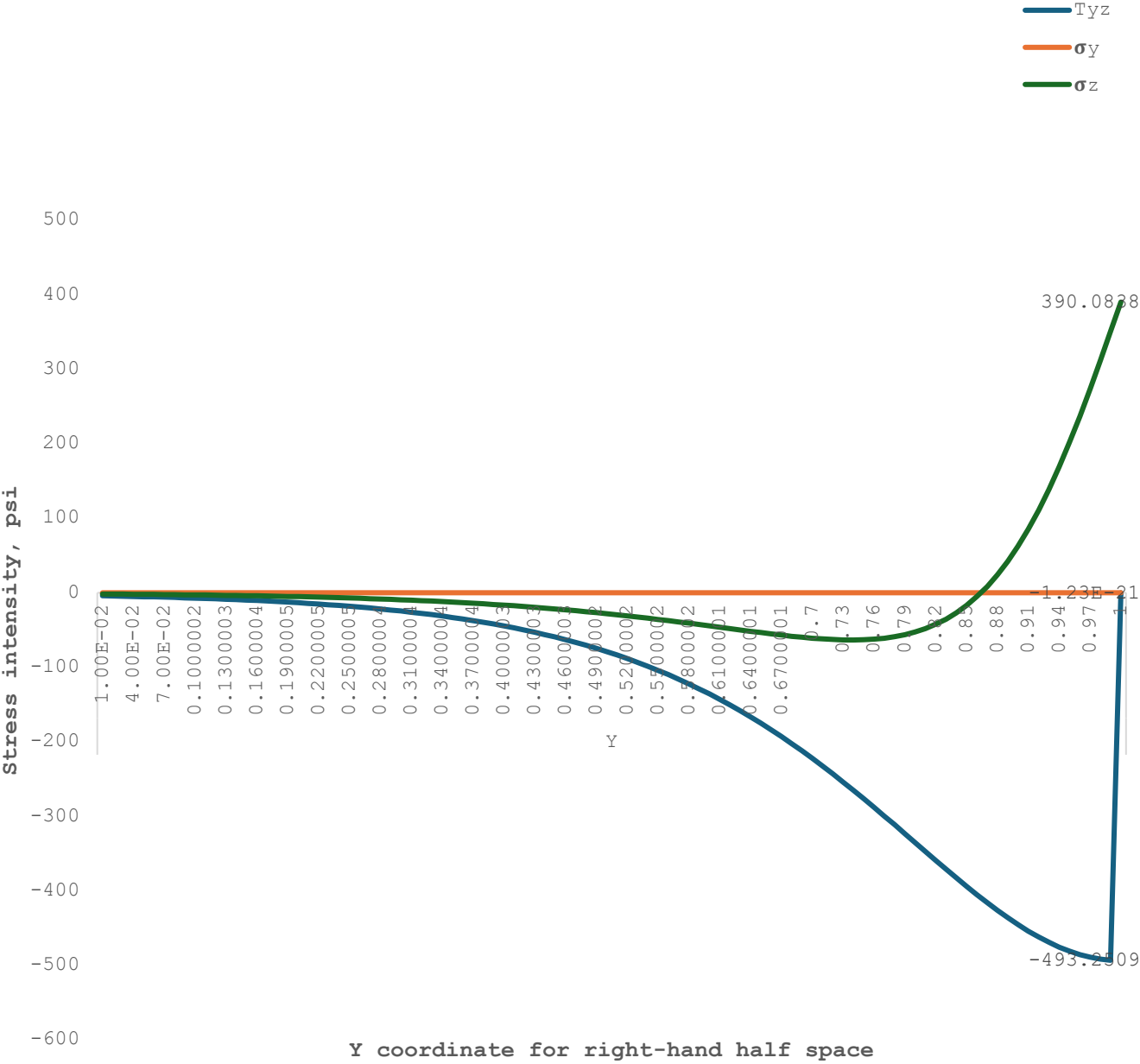
Exact 0/90 Interface at Z=1/2
