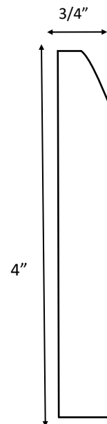
P4 Base Molding
