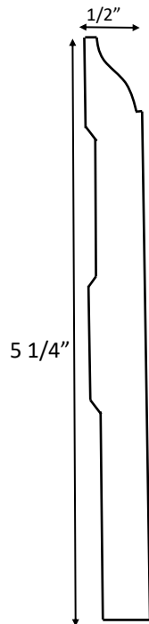
B3 Base Molding
