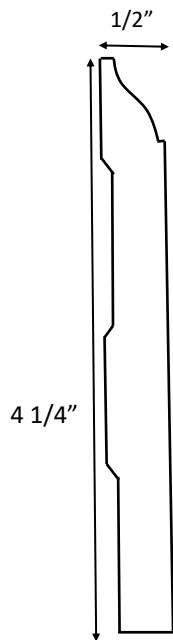
B2 Base Molding
