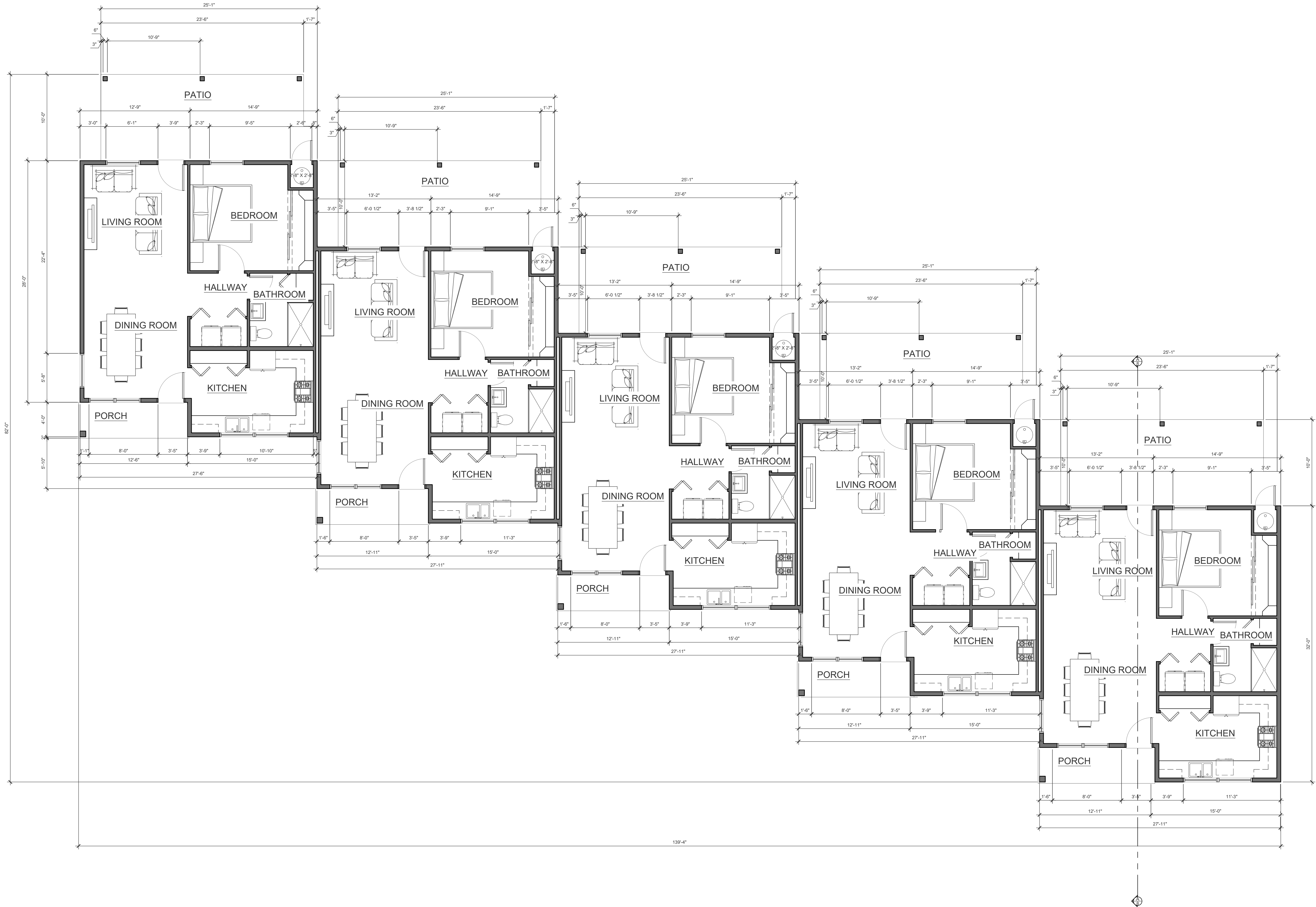
FLOOR DIMENSION PLAN
