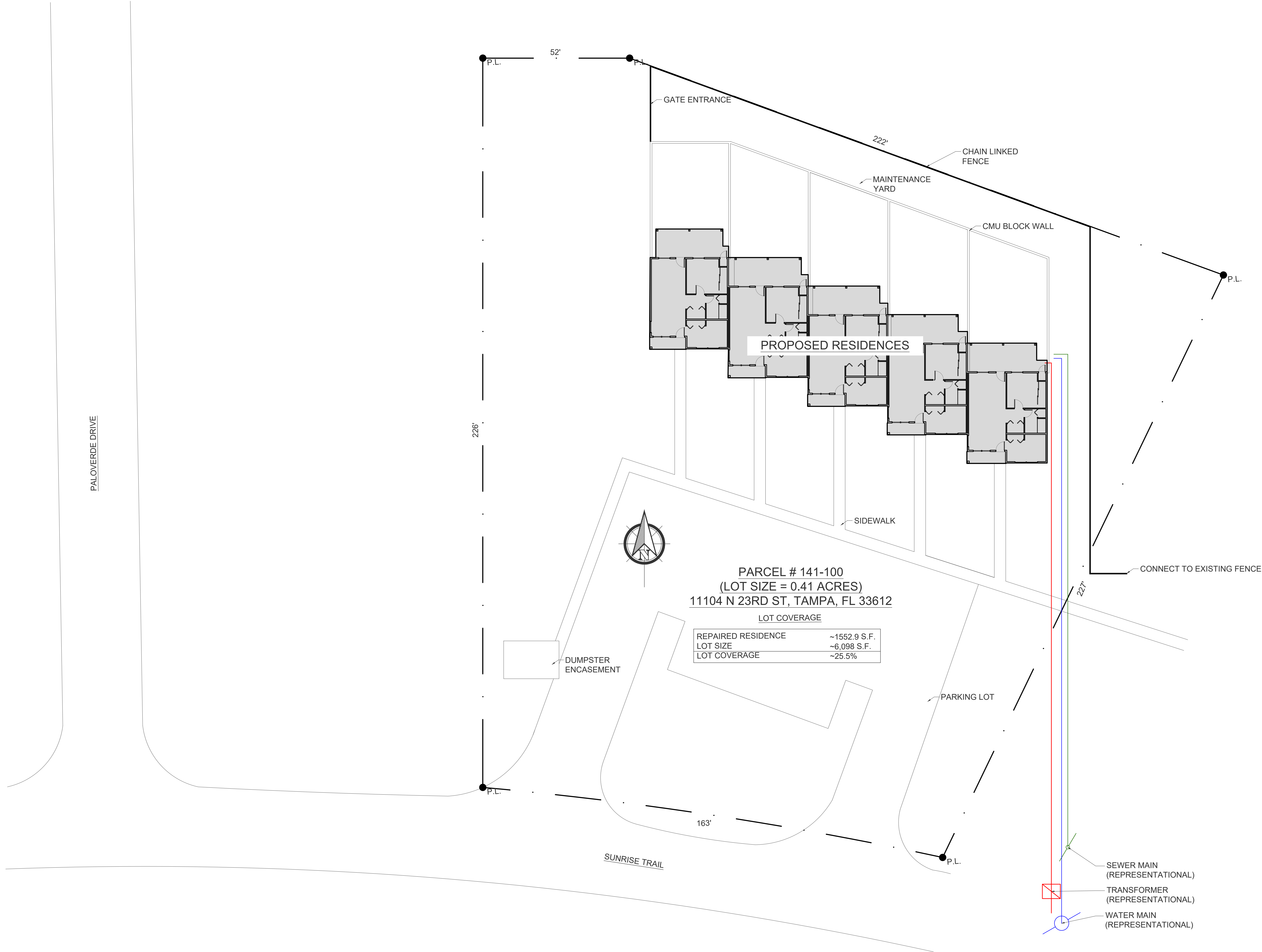
SITE PLAN SCALE: 1/16" = 1'-0"
