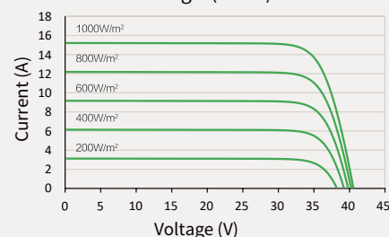
Power-Voltage (500W)
