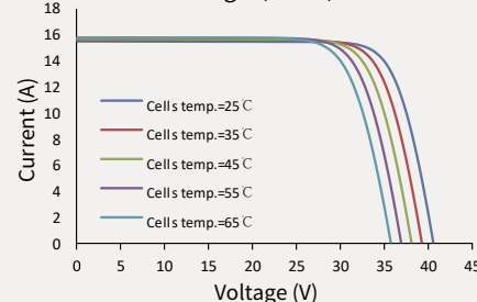
Current-Voltage (500W)
