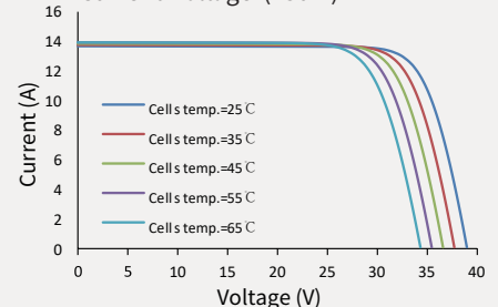
Current-Voltage (430W)
