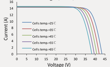
Current-Voltage (485W)
