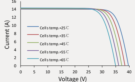
Current-Voltage (440W)
