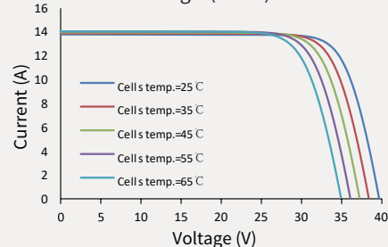
Current-Voltage (435W)
