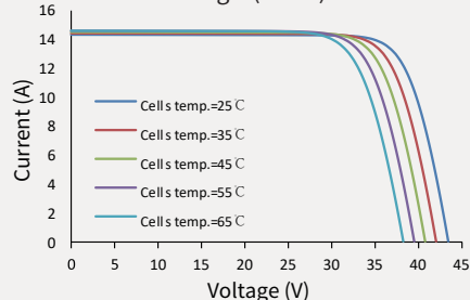
Current-Voltage (485W)
