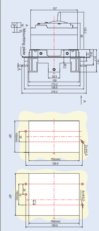
NM8N-250 Plug-in front connection
