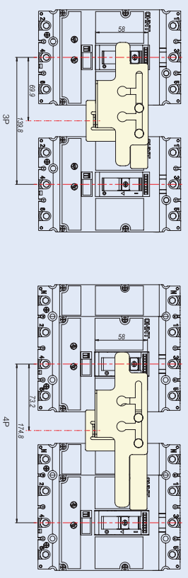
NM8N-250 Mechanical interlock
