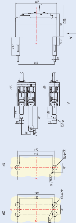
NM8N-250 Rear connection (1P/2P)
