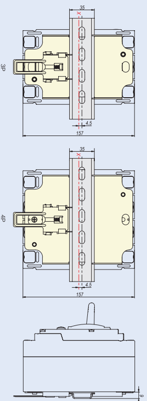
NM8N-250 DIN-rail mounting (DIN-rail adapter is needed)
