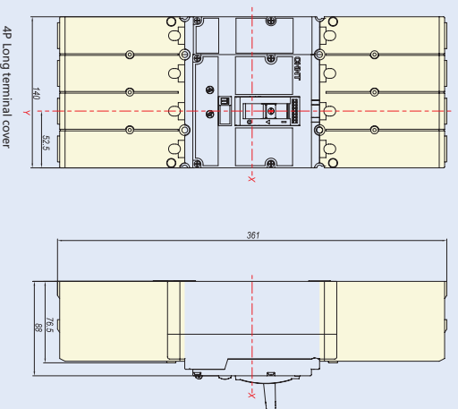
3P Long terminal cover
