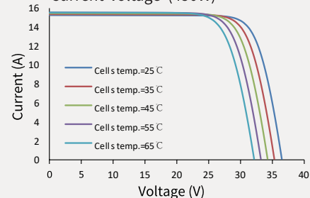
Current-Voltage (450W)
