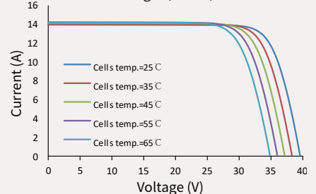
Current-Voltage (440W)
