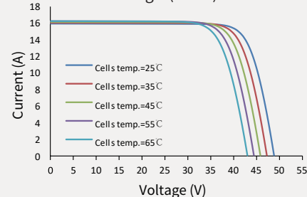
Current-Voltage (615W)
