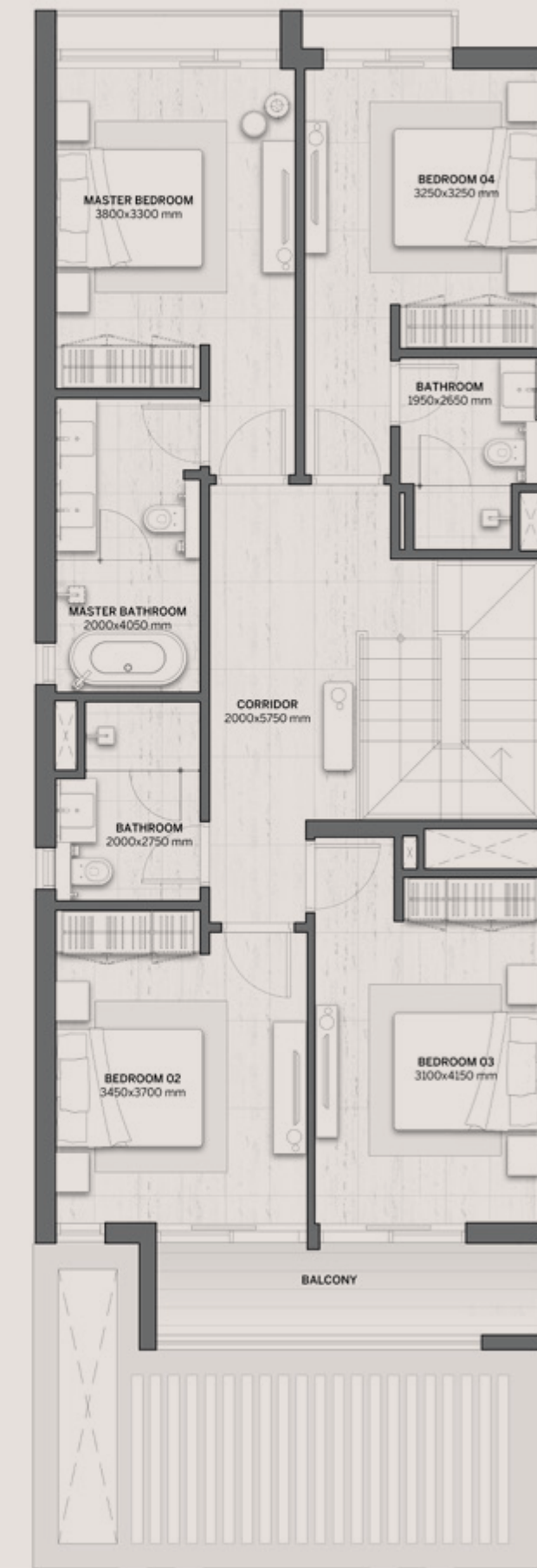
FIRST FLOOR
