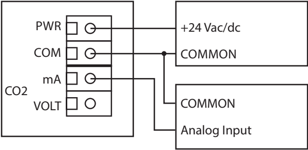
Wiring for 4-20 mA output and external 24 Vac power transformer or power supply
