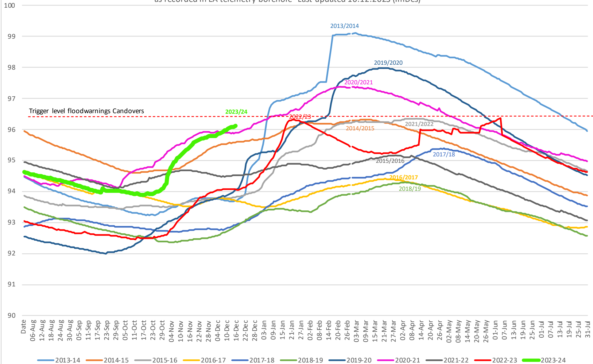
Preston Candover Ground Water Levels - 2013/14 -2023/24 to date as recorded in EA telemetry borehole - Last updated 16.12.2023 (ImDes)
