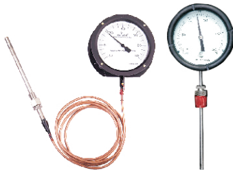
Mercury In Steel
