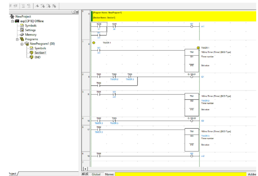
LADDER PROGRAMMING
