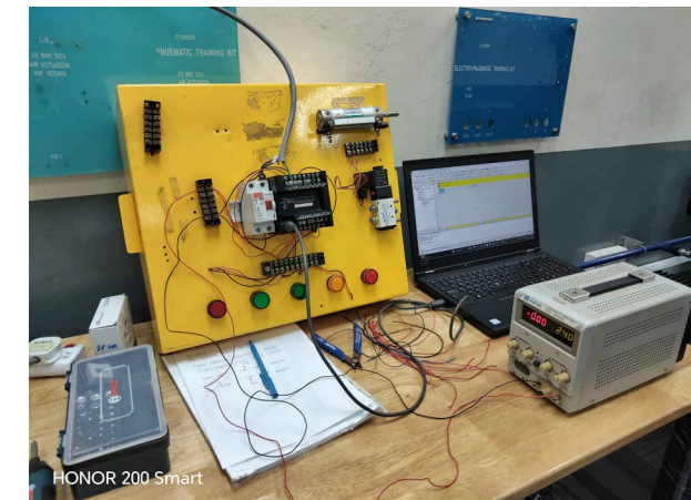
HARDWIRING PRACTICAL
