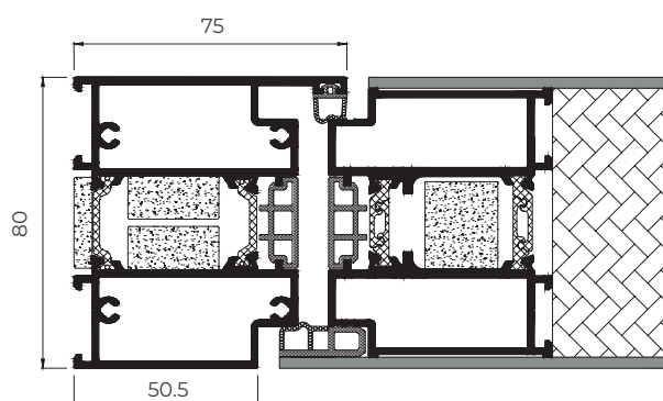
* Panelled version
