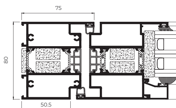
* Glazed version
