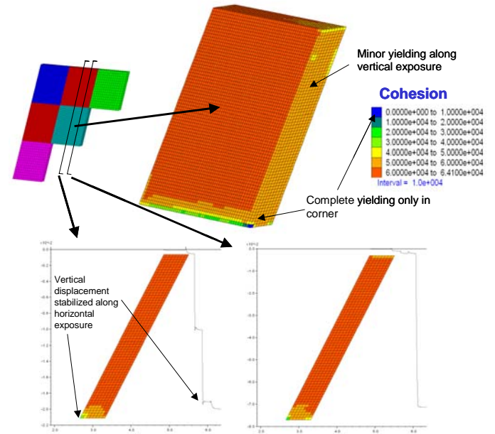
Fig. 18. Significant-yielding classification.
