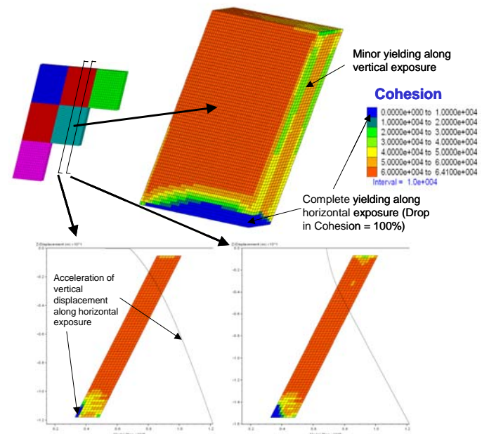
Fig. 19. Crushing-failure classification.
