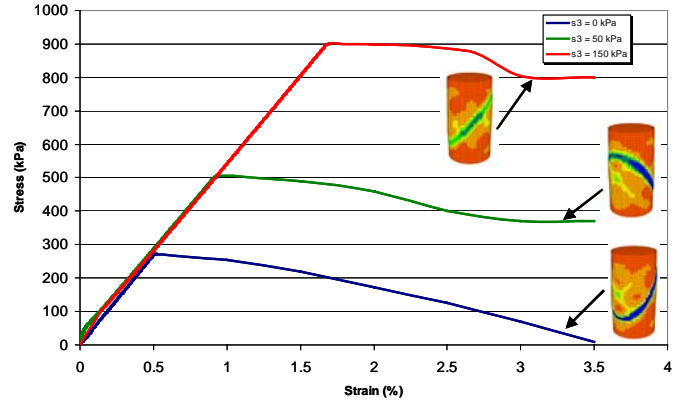
Fig. 12. Calibrated stress – strain response of UCS and triaxial strength test results.
