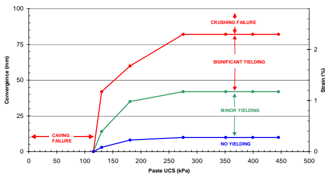
Fig. 21. Stability Chart for 3.5 m wide simultaneous horizontal and vertical exposures.
