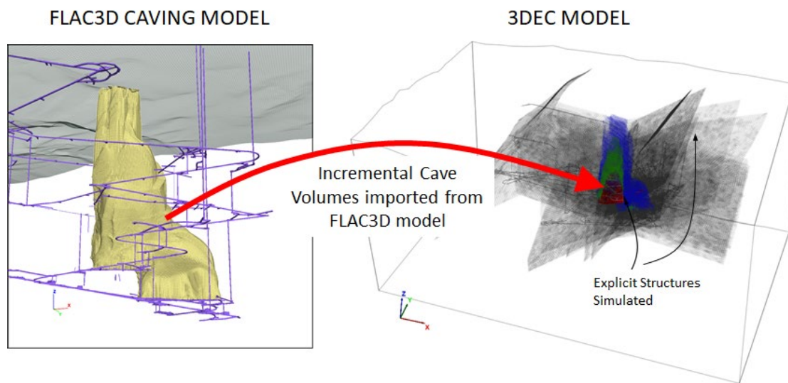
Figure 4 Coupling of FLAC3D and 3DEC models
