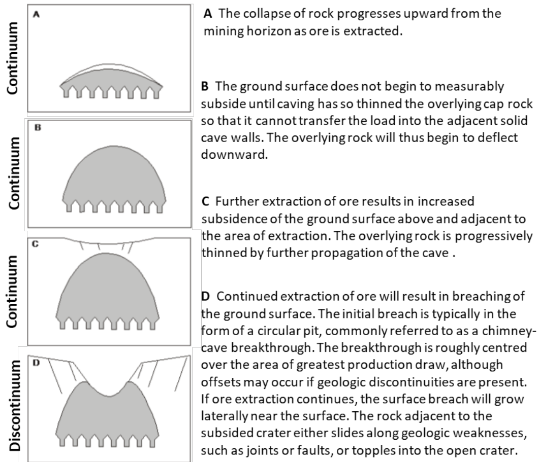
Figure 1 Conceptual model of the development of block caving subsidence (modified after Abel and Lee 1980)
