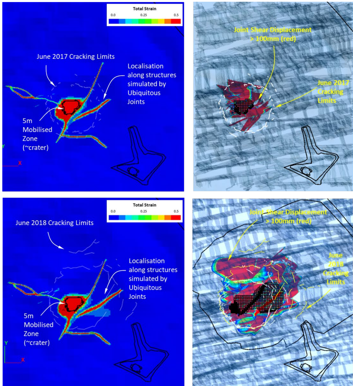
Figure 6 Comparison of existing cracking limits observed and simulated by continuum (left) and discontinuum (right) methods at June 2017 and 2018
