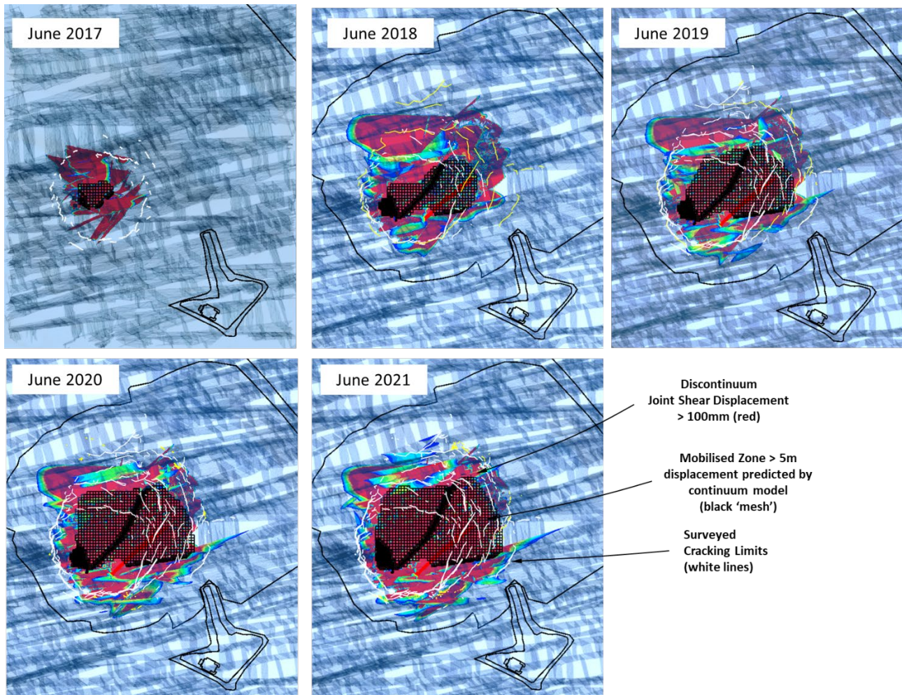
Figure 7 Existing cracking limits observed and simulated by discontinuum from June 2017 - June 2021
