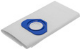
Filter bag, fleece for S-series and C-series size: 490 x 640 mm Item # 13060
