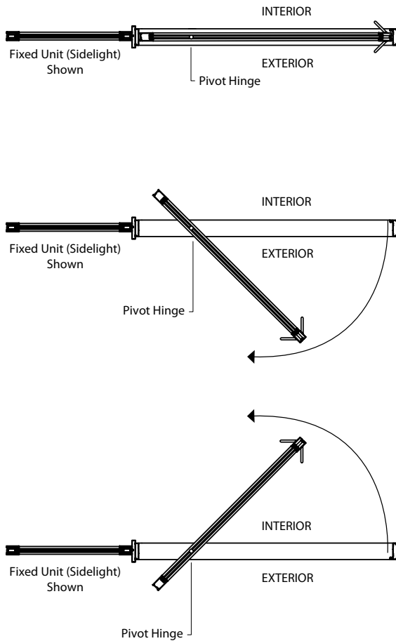
TOP VIEW - Horizontal Cross Section
