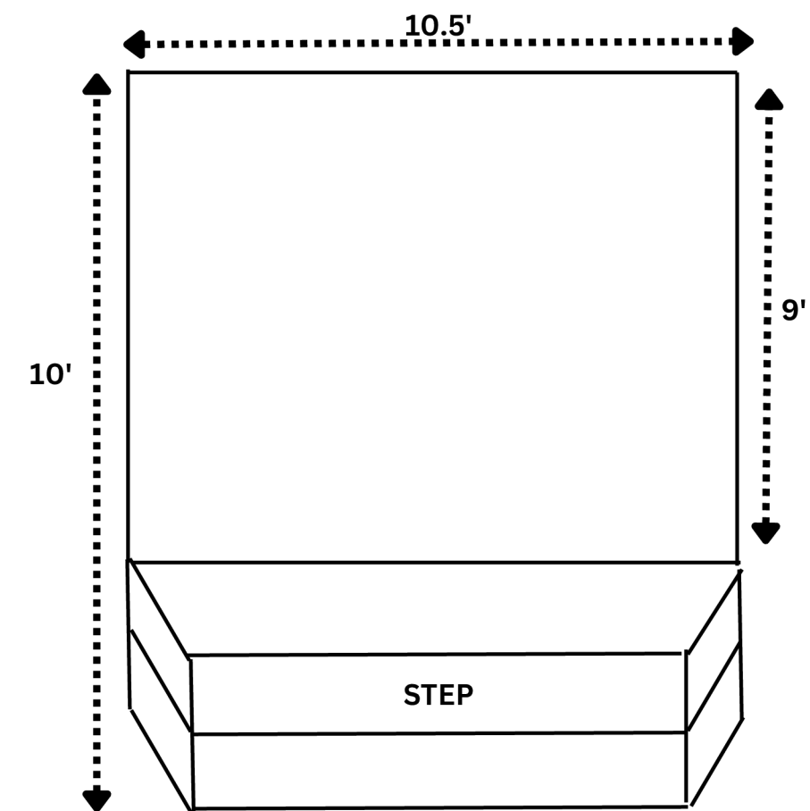
BASE/STAGE
