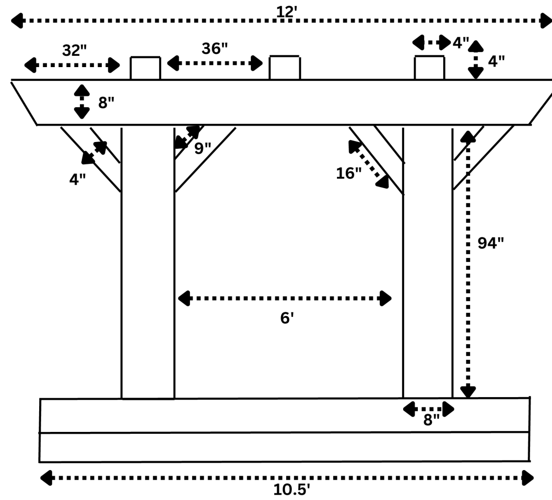
FRONT
