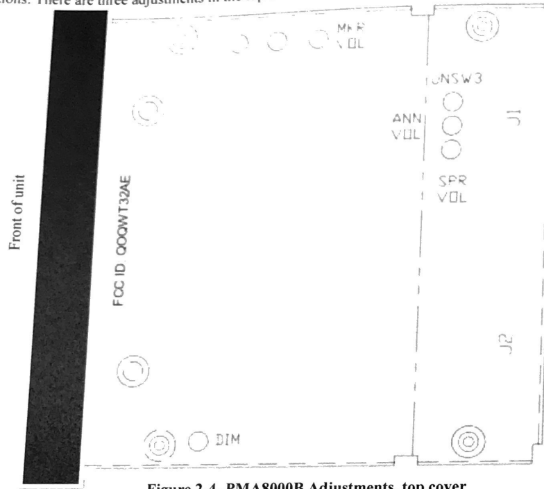
Figure 2-4- PMA8000B Adjustments, top cover
