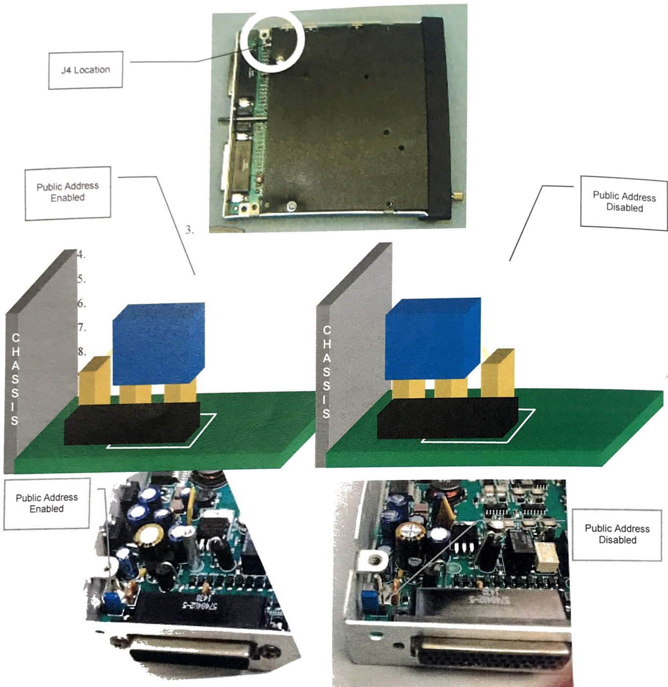
Figure 2-3 Jumper Location
