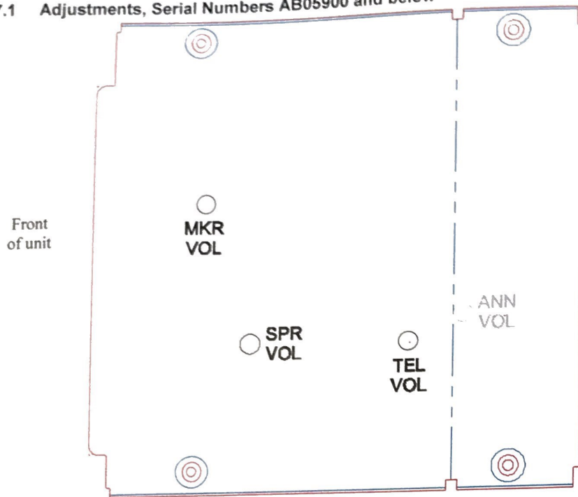
Figure 2-5- PMA8000B Adjustments, top cover
