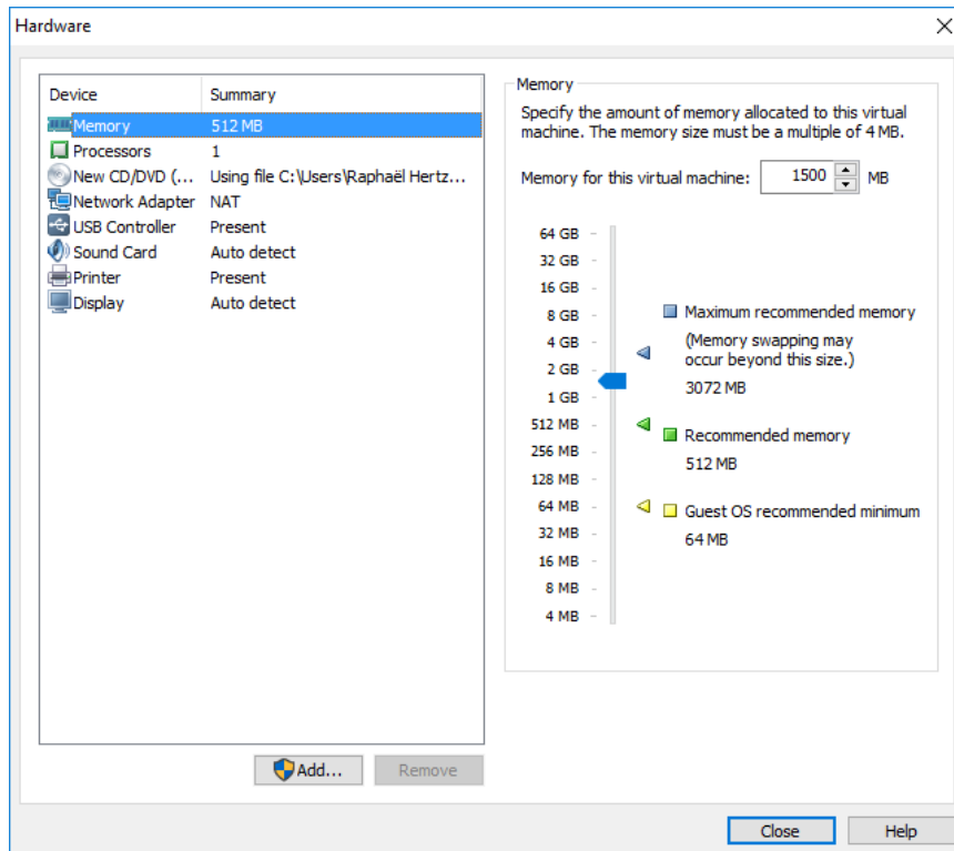
Figure 2.25 Configure Hardware Window
