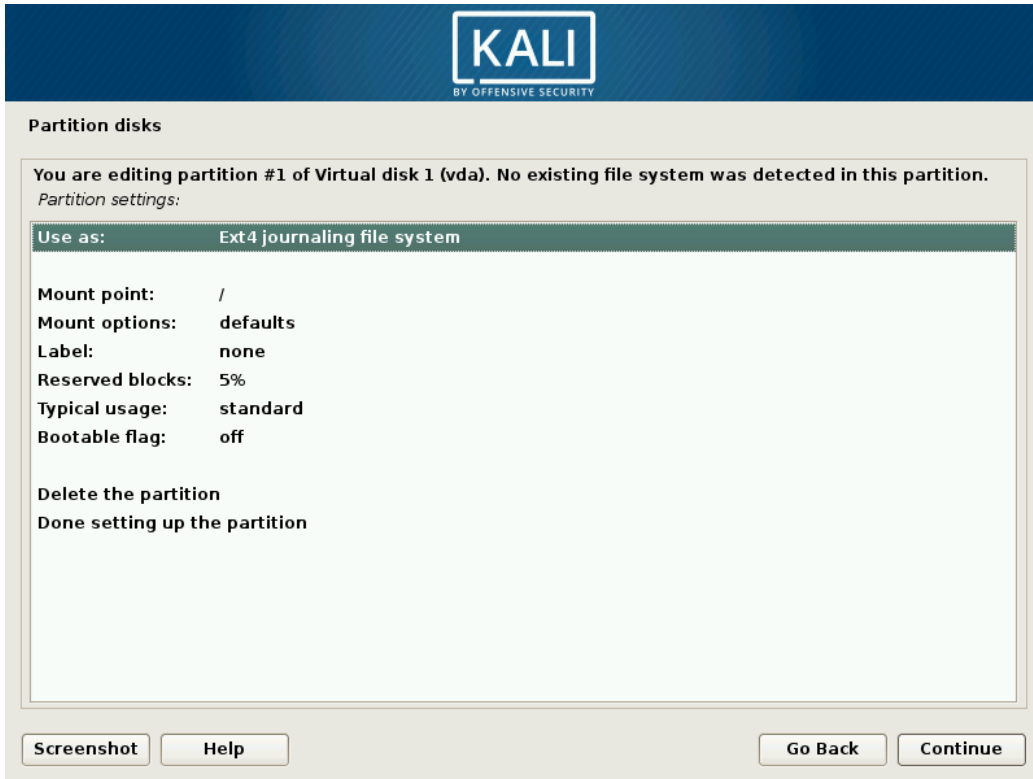
Figure 4.13 Partition Configuration Screen
