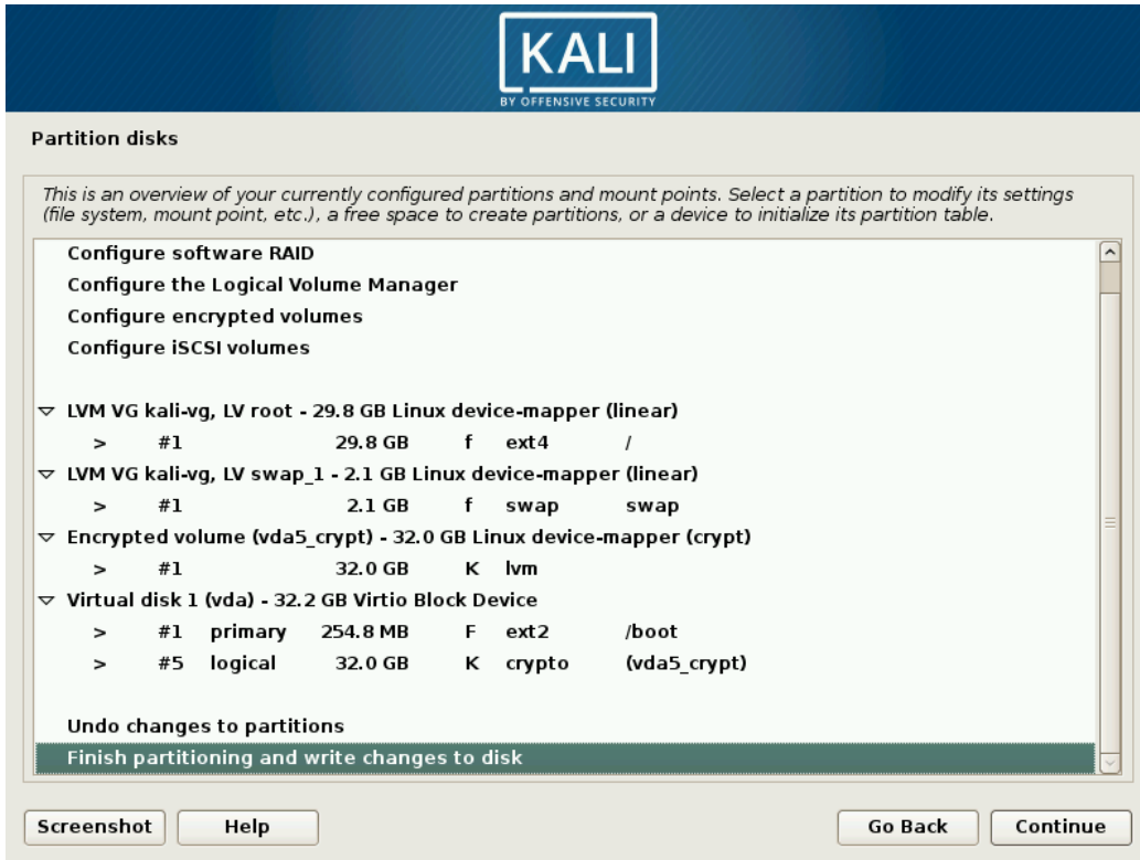
Figure 4.24 Validating Partitioning for Encrypted LVM Installation
