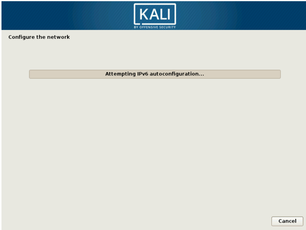
Figure 4.5 Network Autoconfiguration
