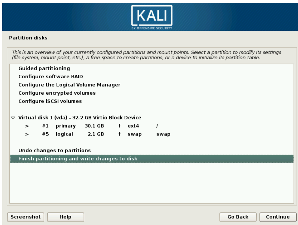
Figure 4.11 Validating Partitioning
