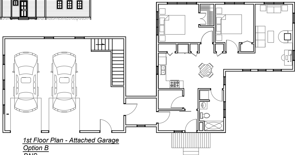
GRAY BIRCH - Attached Garage Option B DNS
