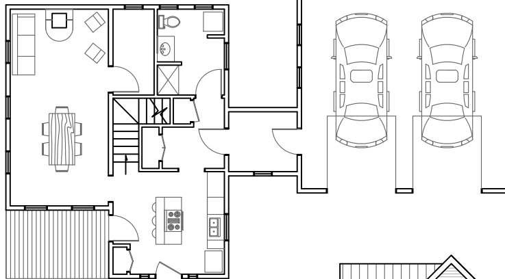
1st Floor Plan - Attached Garage Option A DNS
