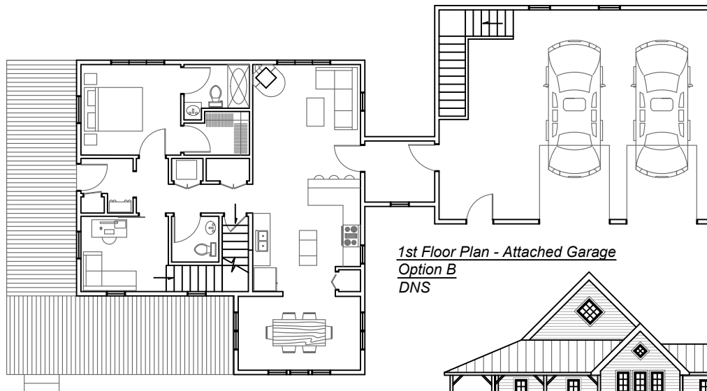
WHITE OAK - Attached Garage Option B DNS
