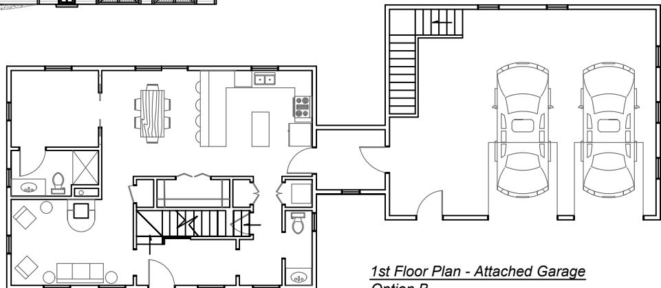
MAPLE - Attached Garage Option B DNS
