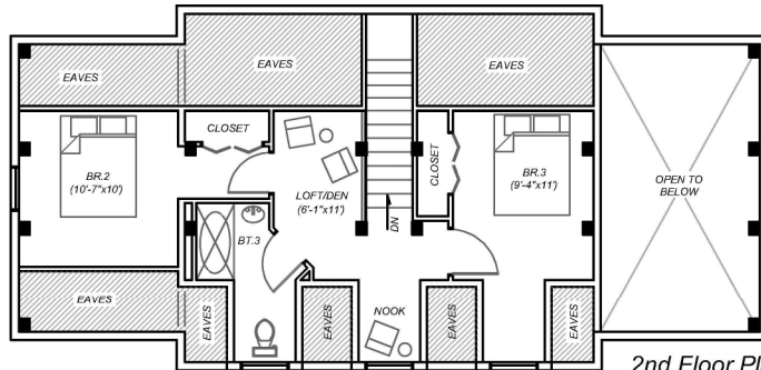
2nd Floor Plan DNS
