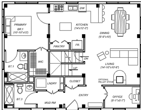
1st Floor Plan DNS
