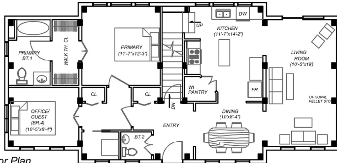
1st Floor Plan DNS
