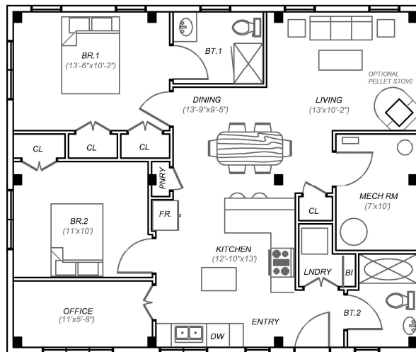
1st Floor Plan DNS
