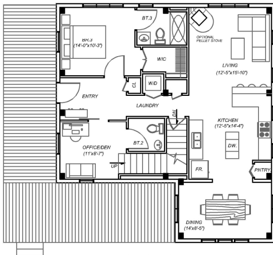
1st Floor Plan DNS
