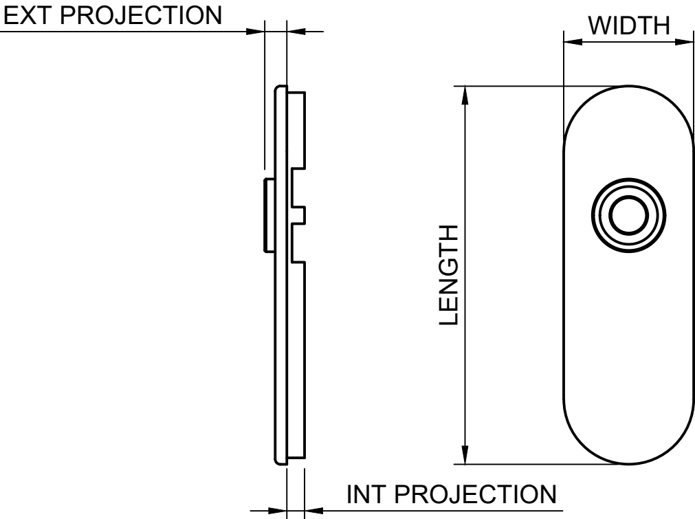
SIXTA LEVER HANDLE 145 BACKING PLATE
