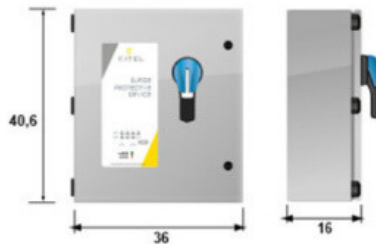
MDS600E series
