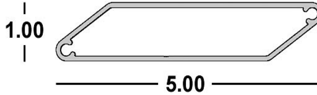
Shadow Box Panel 5" x 24'
