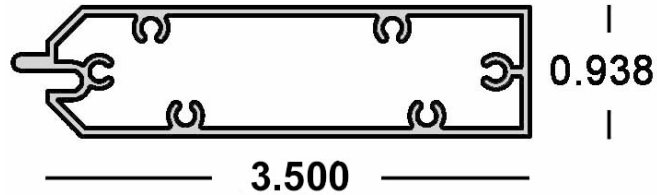
Tongue & Groove Starter 0.938" x 3.5" x 24'
