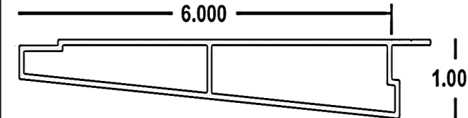
Hardy Plank 6" x 24'
