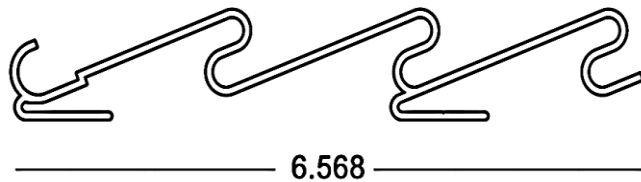
2" Fixed Bahama Triple Blade x 12' SELF MATING
