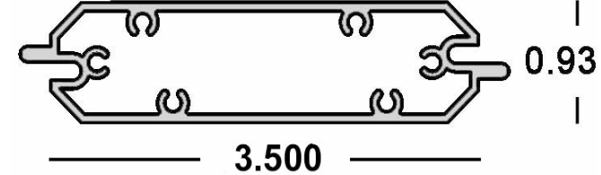
Tongue & Groove Starter SELF MATING - 0.938" x 3.5" x 24'
