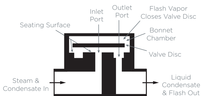
Figure 9. Thermodynamic Disc Steam Trap
