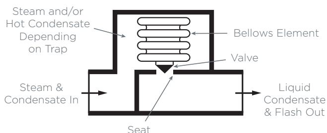
Figure 5. Thermostatic Steam Trap with a Bellows Element
