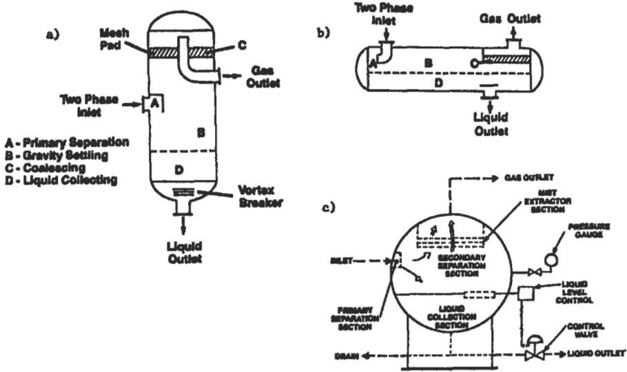
Figure 6-179. Gas liquid separators: (a) vertical, (b) horizontal, (c) spherical [117].
