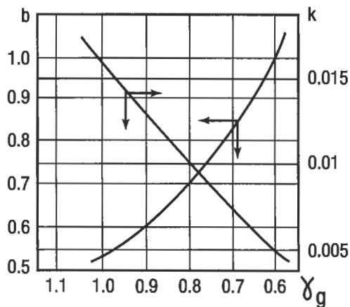
Figure 6-206. Dependence of coefficients \beta and k on the relative density ( SG_g ) [133].
