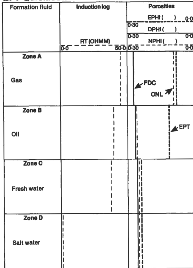
Figure 5-106. EPT quicklook chart comparing curve response of induction resistivity, neutron porosity, density porosity and EPT porosity in water bearing and hydrocarbon-bearing zones [214].
