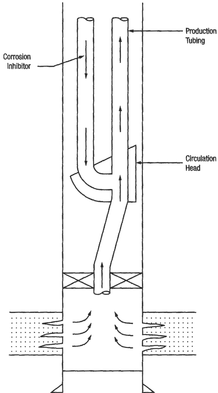
Figure 6-253. Y-block completion [184].
