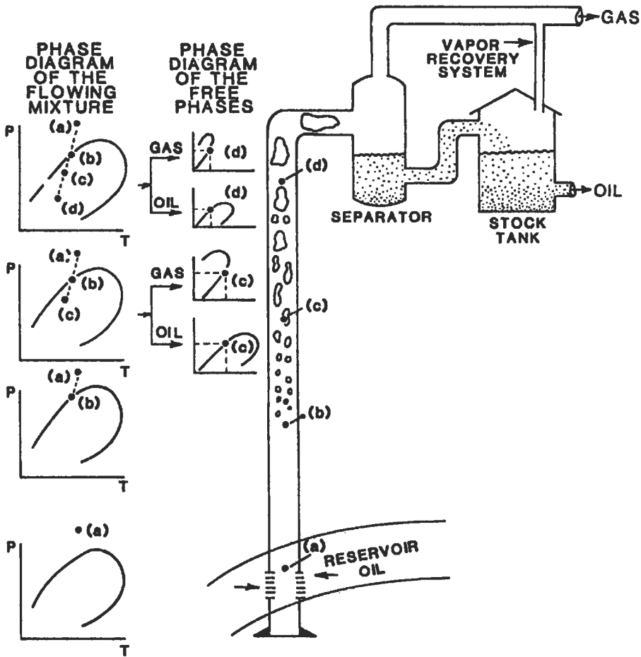
Figure 6-39. Changes in phase behavior in the production tubing [20].
