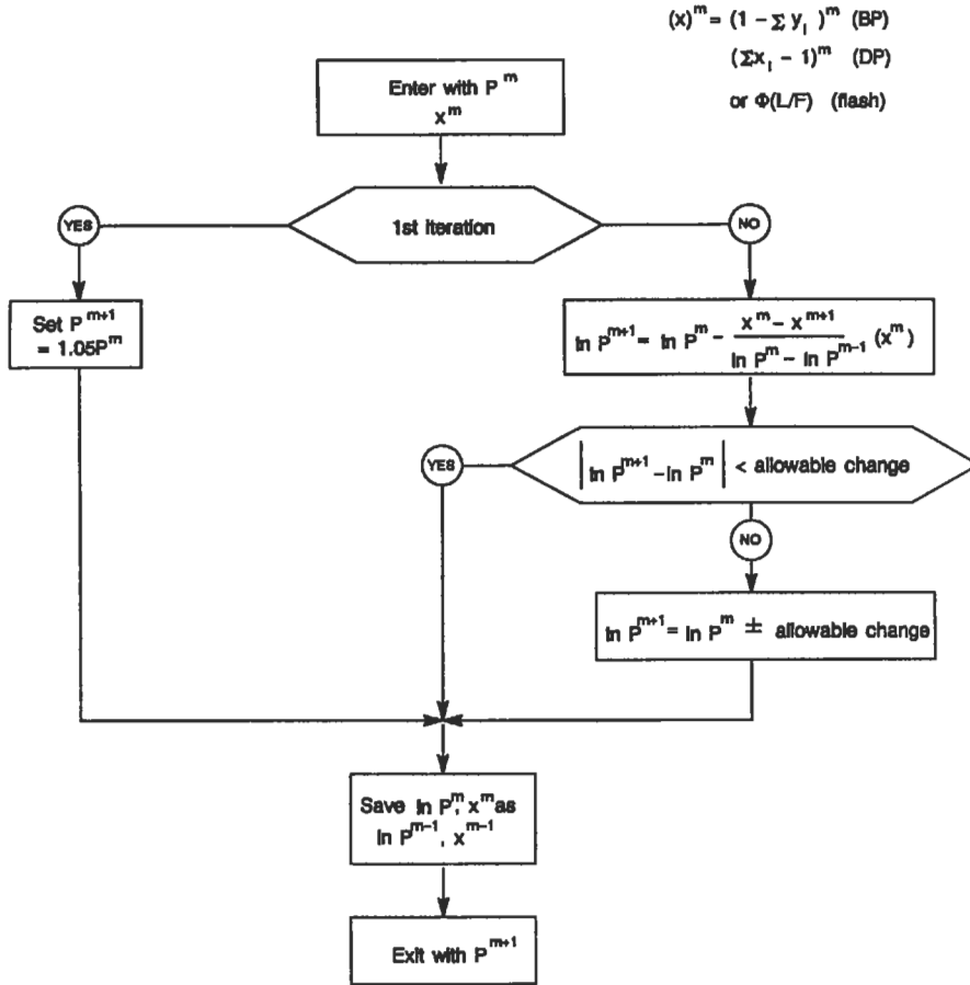
Figure 6-27. Pressure adjustment diagram for equilibrium calculations.
