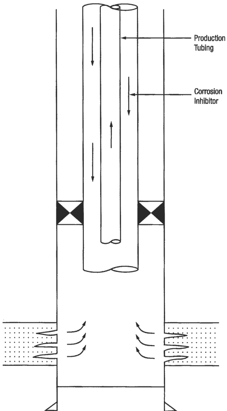
Figure 6-252. Concentric completion [184].
