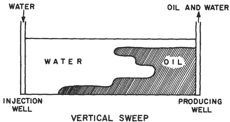
Figure 5-158. Sweep efficiencies.
