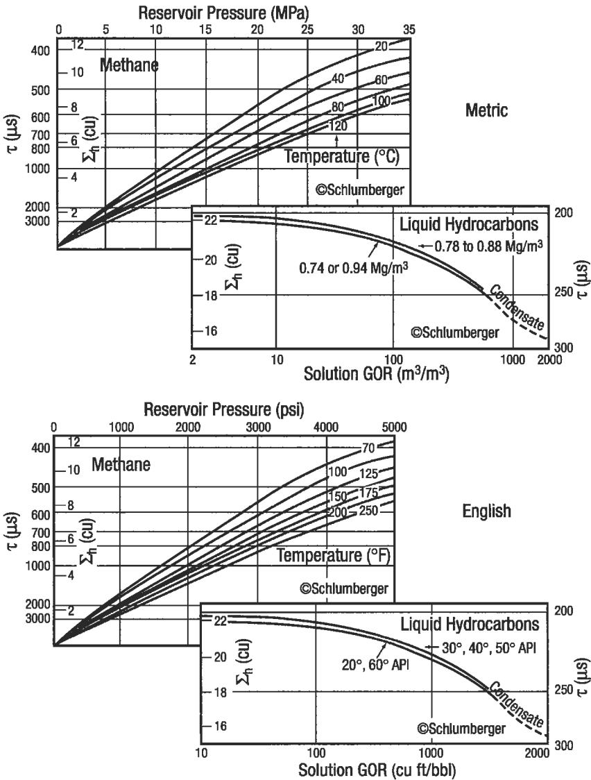
Figure 5-113. Charts for finding \Sigma_h (for methane and liquid hydrocarbons) from reservoir pressure and formation temperature (gas) or solution gas oil-ratio (GOR) and API gravity (liquid 7 hydrocarbons [199]).
