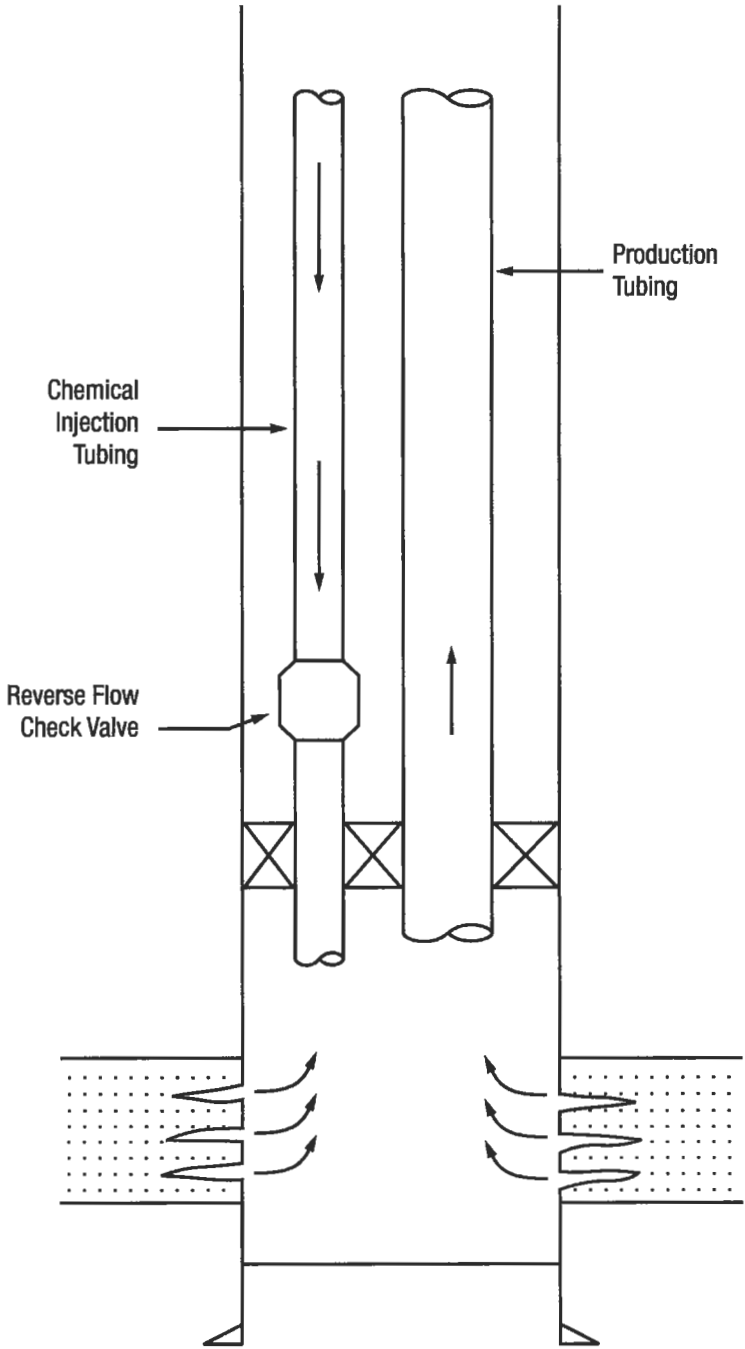
Figure 6-251. Dual completion [184].
