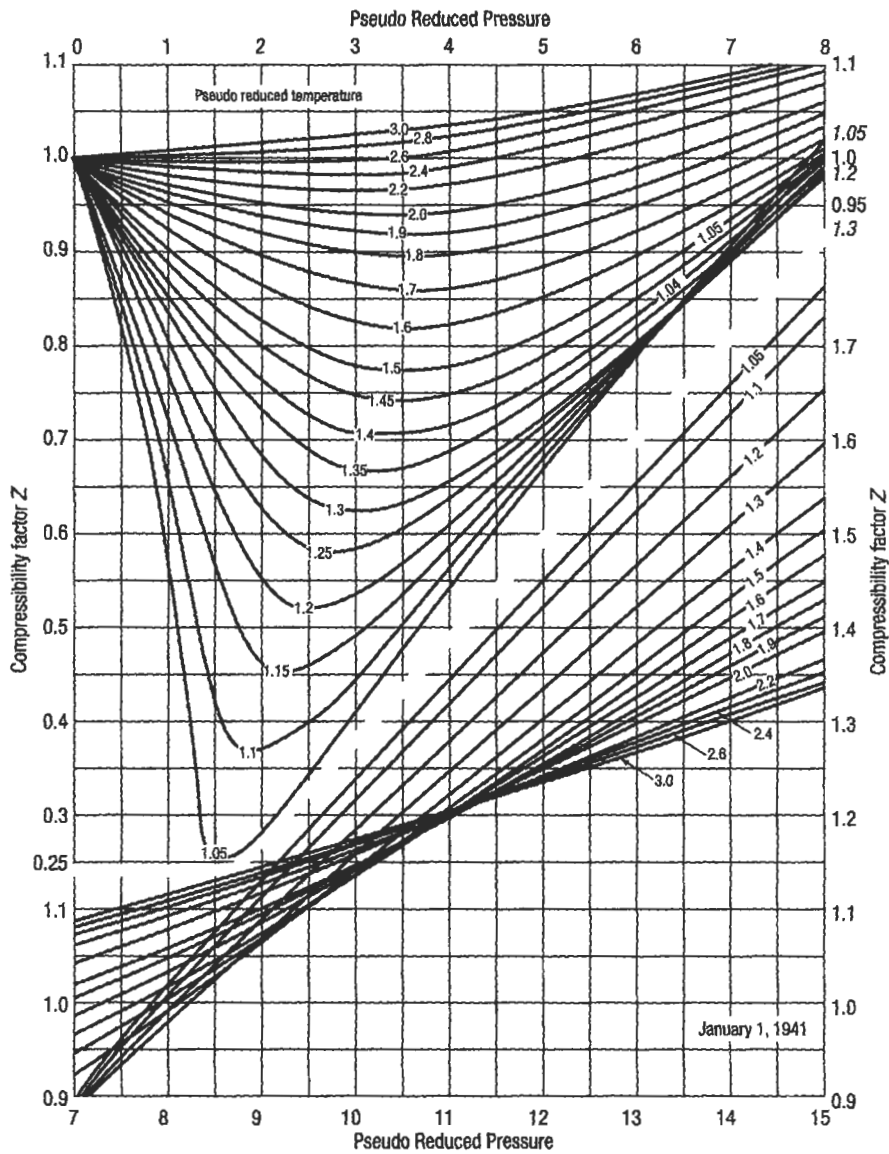
Figure 6-1. Compressibility factor for natural gases [1].
