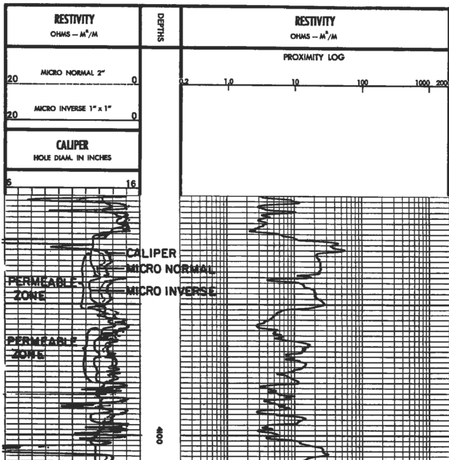
Figure 5-87. Example log showing positive separation of the microlog curves opposite a permeable formation at 4,030 to 4,050 feet.
