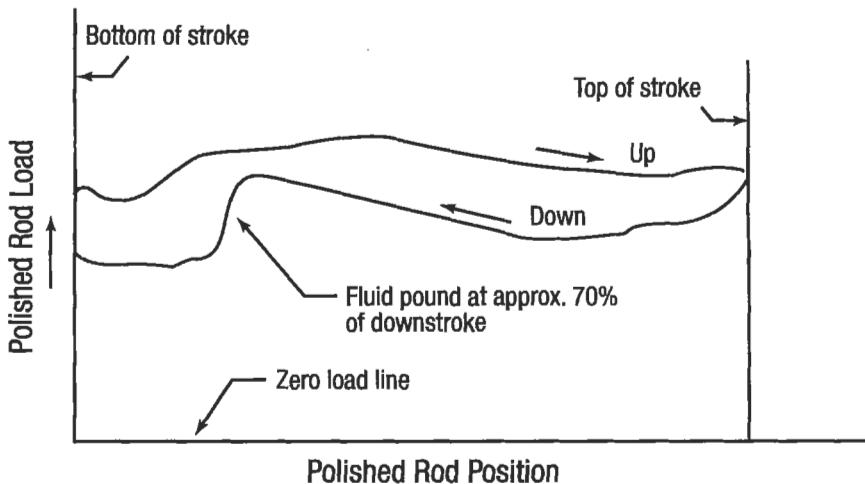
Figure 6-131. Example of fluid pound [68].
