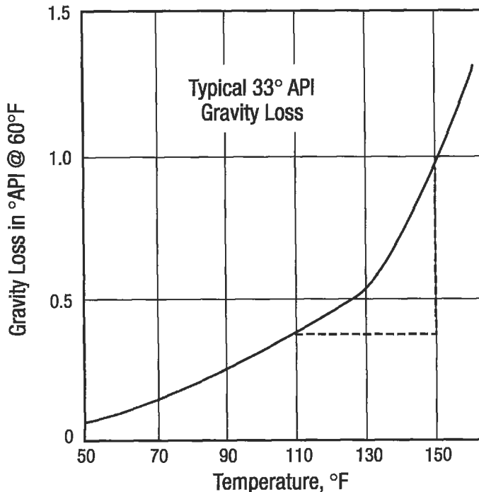
Figure 6-190. API gravity loss vs. temperature for crude oil [126].
