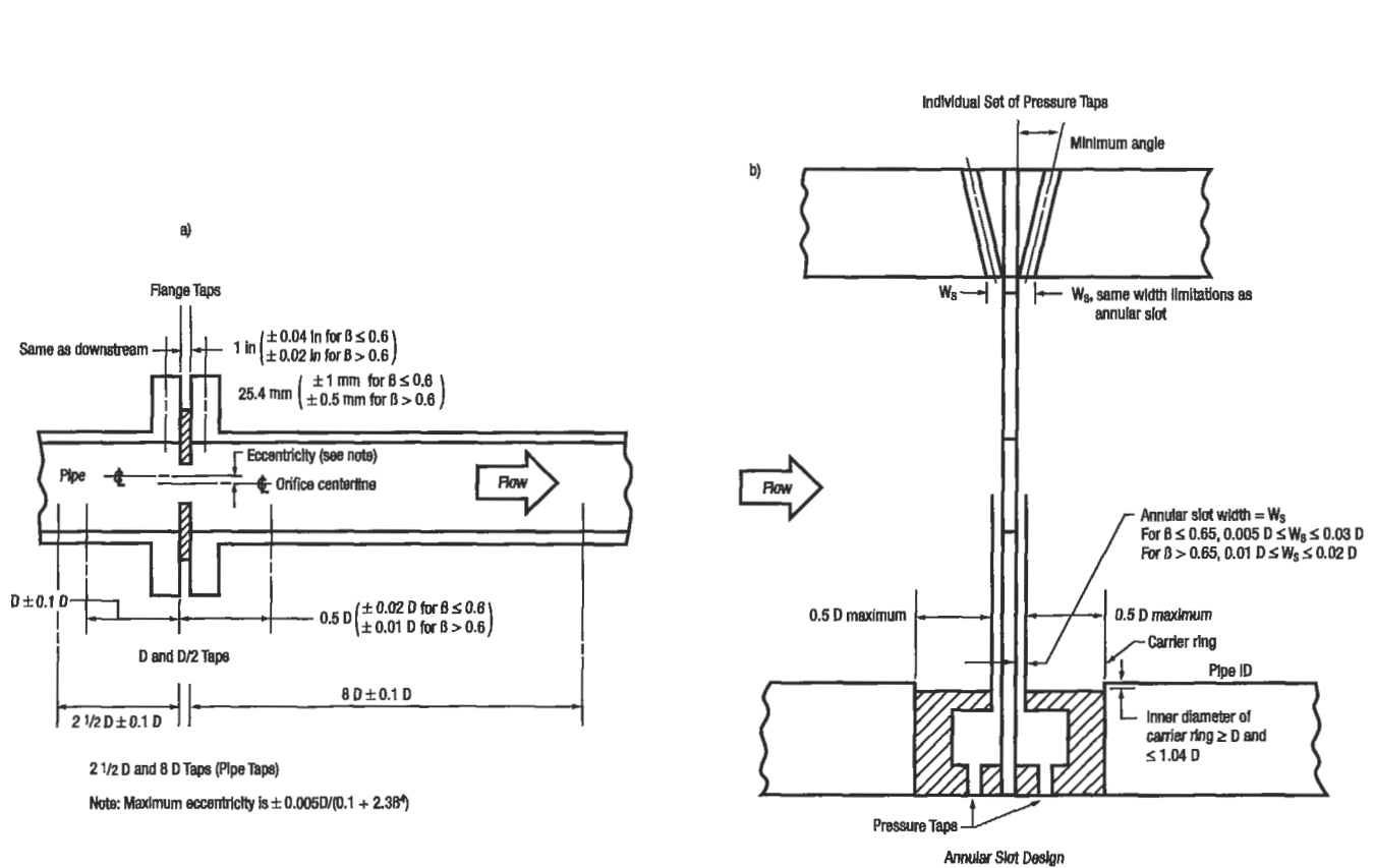
Figure 6-224. Pressure-tap spacing [141].
