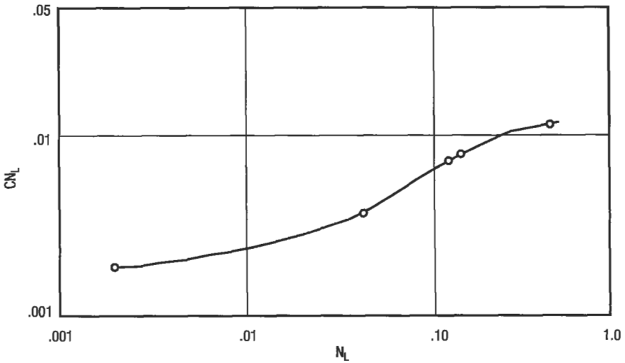
Figure 6-73. Correlation for viscosity number coefficient [29].
