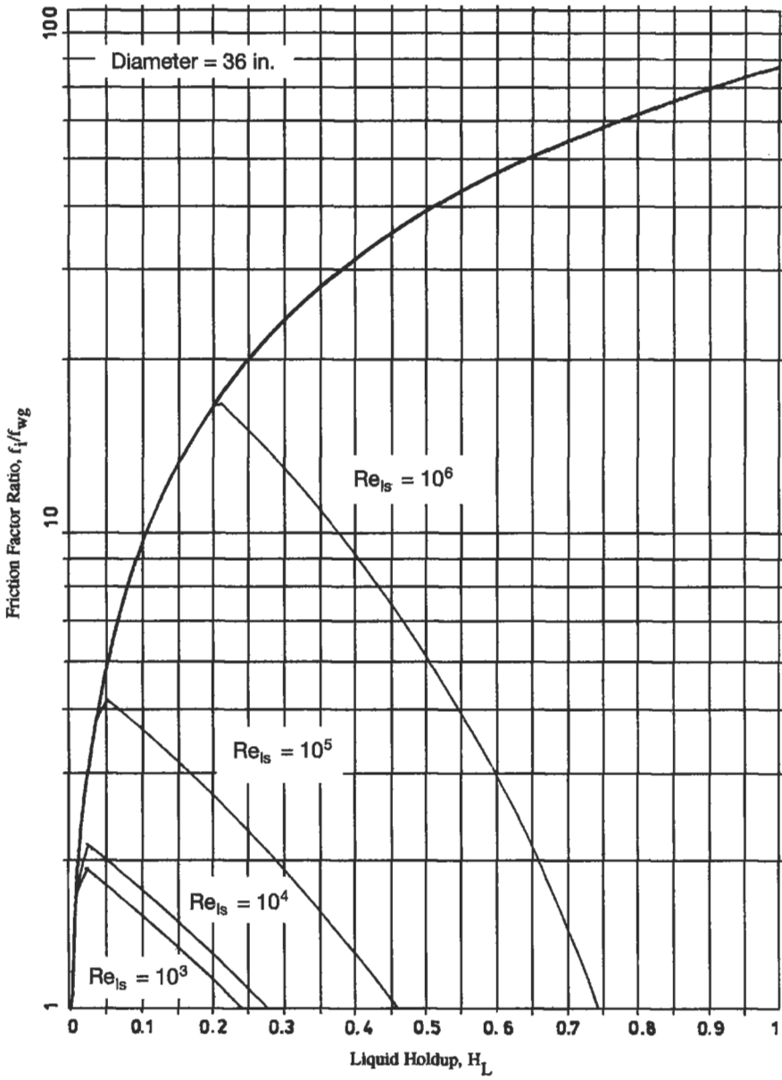
Figure 6-48h. Interfacial friction factor ratio for stratified flow regime (D = 36 inches) [22].
