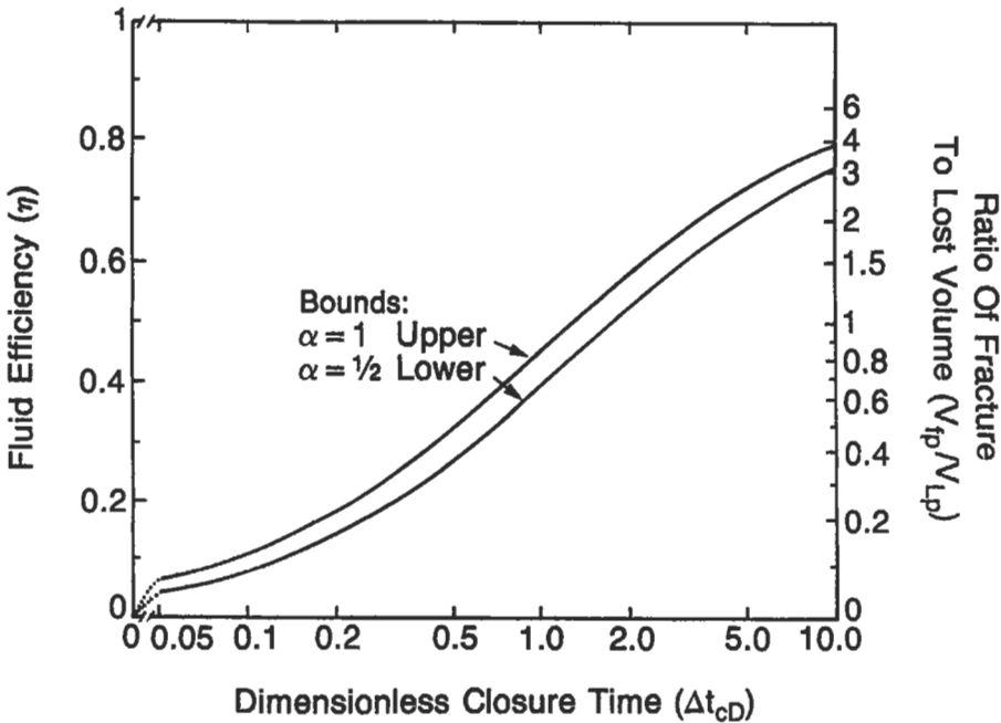
Figure 6-152. Fracturing fluid efficiency correlation. The dimensionless closure time \Delta t_{cD} is the ratio of the closure time to the pumping time [79].
