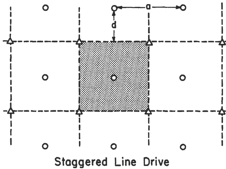
Figure 5-152. Distances in line drive patterns [25].
