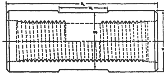
POLISHED-ROD COUPLING
