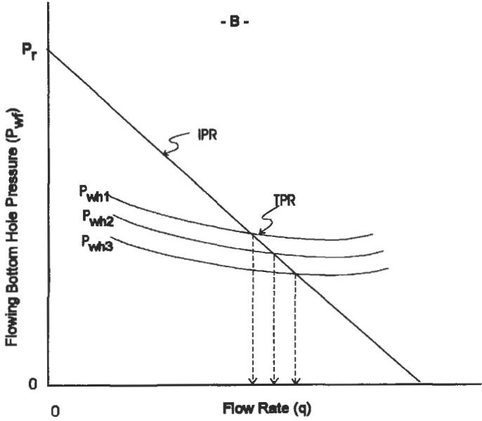
Figure 6-78. Effects of tubing size and tubing head pressure on a well productivity.
