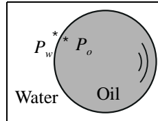
Figure 6.4: Pressure difference across a curved (spherical) interface.
