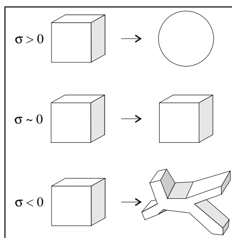
Figure 6.6: Formation of interface as function of the sign of the interfacial tension in pairs of immiscible unconfined fluids.
