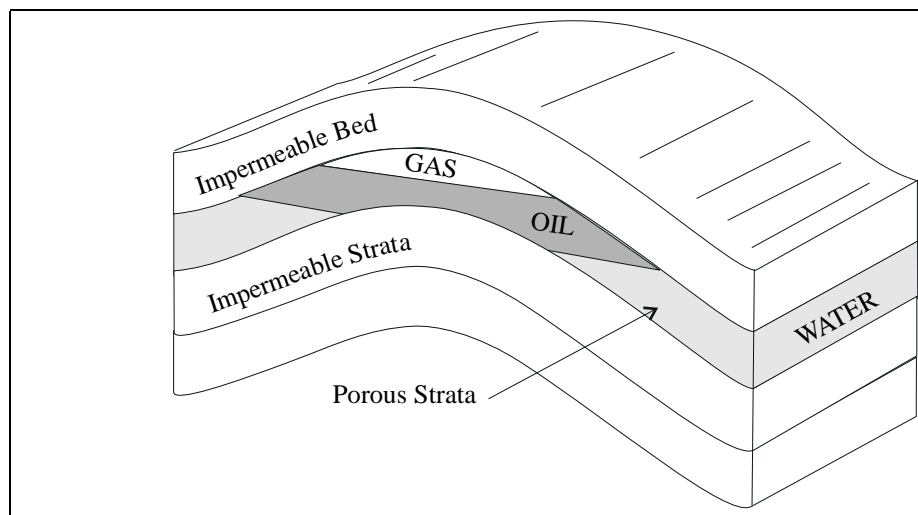
Figure 2.6: Oil and gas accumulation in an anticline structure.
