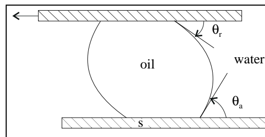
Figure 6.18: Measurement of hysteresis in contact angle.
