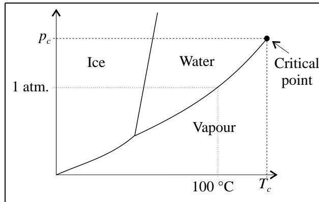
Figure 9.2: PT-diagram for H_2O .
