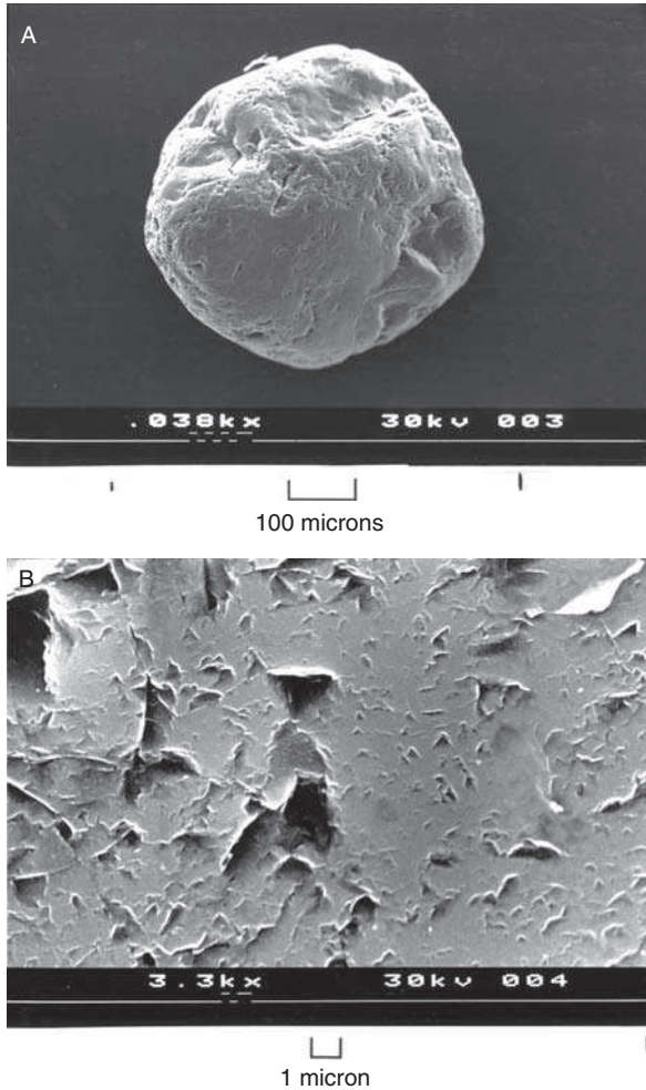
Figure 2.18 A. Electron micrograph of surface markings on a quartz grain from a late Pleistocene high-energy beach deposit near Norwich, Norfolk, England. B. Enlarged portion of the extreme right edge of the grain in A. Note abundant V-shaped markings, which are characteristics of quartz grains from high-energy beaches. [Photograph courtesy of David Krinsley.]
