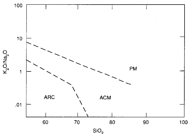
Figure 7.13 Chemical model for discriminating tectonic setting of sandstones and argillites on the basis of K_2O/Na_2O ratios and SiO_2 content. ARC = oceanic-island-arc margin, ACM = active continental margin, PM = passive margin. (After Roser, B. P. and R. J. Korsch, 1986, Determination of tectonic setting of sandstone–mudstone suites using SiO_2 content and K_2O/Na_2O ratios: J. Geol. , 94 , Fig. 2, p. 638, reprinted by permission of University of Chicago Press.)
