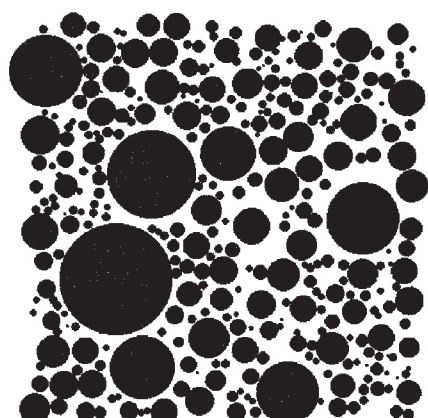
Figure 2.3 Textural comparison chart showing degree of sorting. Each section is labeled with its verbal sorting description according to Folk (1968). (After Jerram (2001), Visual comparators for degree of grain-size sorting in two and three-dimensions: Comput. Geosci. , 27, Fig. 5, p. 490. Reproduced by permission of Pergamon Press, Elsevier Science Ltd.)
