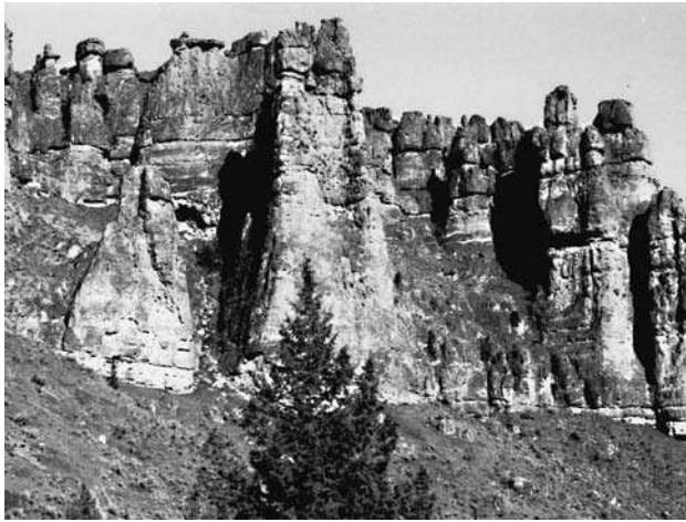
Figure 5.14 Massive to crudely stratified subaerial debris-flow conglomerate. Clarno Formation (Eocene–Oligocene), eastern Oregon. (Photograph courtesy of G. J. Retallack.)
