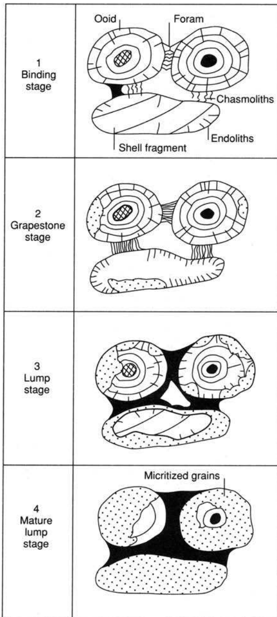
Figure 9.17 Stages in the formation of aggregate grains. Stage 1: carbonate grains are bound together by foraminifers, microbial filaments, and mucilage. Chasmolitic microorganisms occur between the grains, whereas endolithic forms bore into the carbonate substrates. Stage 2: calcification of the microbial braces occurs, typically by high-magnesian calcite, to form a cemented grapestone. Progressive micritization (conversion to lime mud) of carbonate grains takes place. Stage 3: increased cementation at grain contacts, by microbially induced precipitation, fills depressions to create smoother relief. Stage 4: filling of any central cavity to form a dense, heavily micritized and matrix-rich aggregate. Some replacement of the high-magnesian calcite components by aragonite may also occur. (After Tucker, M. E. and V.P. Wright, 1990, Carbonate Sedimentology : Blackwell Scientific, Oxford, Fig. 1.8, p. 12, reproduced by permission.)
