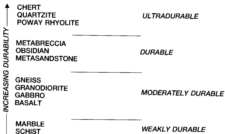
Figure 7.15 Abrasional durability scale for clasts. (From Abbott, P.L., and G.L. Peterson, 1978, Effect of abrasion durability on conglomerate clast populations: examples from Cretaceous and
