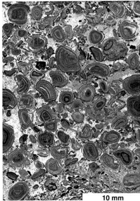
Figure 9.14 Nonmarine pisolites from the vadose zone (vadoids), Upper Triassic, Croatia. [From Peryt, T. M., 1983, Vadoids , in Peryt, T. M. (ed.), Coated Grains , Springer-Verlag, Berlin, Fig. 2, p. 441, reproduced by permission.]
