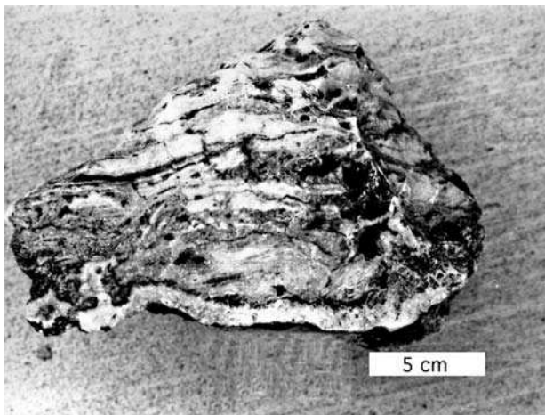
Figure 9.41 Crudely banded travertine. Unknown location. (Specimen furnished by R. A. Linder.)
