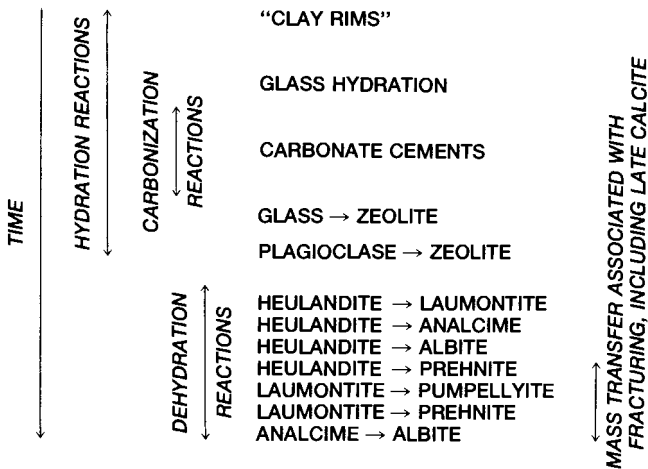
Figure 8.20 Descriptive framework for zeolitization and other diagenetic changes in volcanoclastic sediments. (From Surdam, R.C. and J.R. Boles, 1979, Aspects of Diagenesis : SEPM Special Publication 26, Fig. 17, p. 241, reprinted by permission of the Society for Sedimentary Geology, Tulsa, OK).
