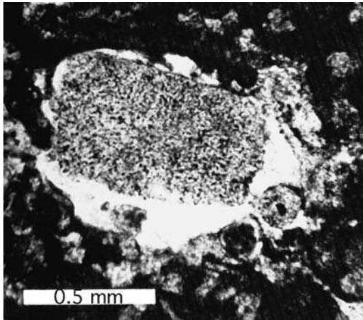
Figure 11.19 Syntaxial overgrowth (bright) surrounding a large crinoid grain. Plane-light photomicrograph. (Modified from Walkden, G. M., and J. R. Berry, 1984, Syntaxial overgrowths in muddy crinoidal limestones: cathodoluminescence sheds new light on an old problem: Sedimentology , 31 , Fig. 2, p. 253, reproduced by permission of Blackwell Publishing, Inc.)
