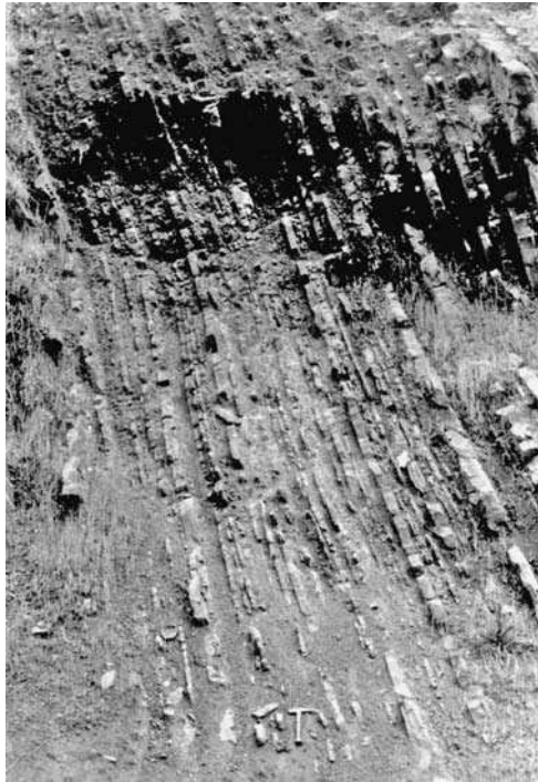
Figure 4.22 Rhythmic bedding in thin, graded lithic arenites of the Roseburg Formation (Eocene), southern Oregon Coast Range. The beds are tilted at an angle of about 70 degrees. Note the hammer for scale.
