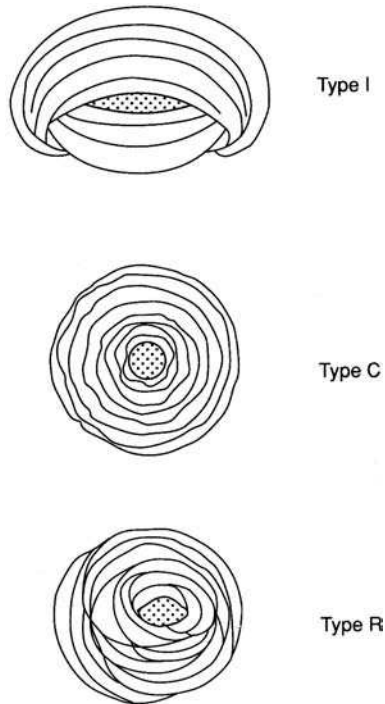
Figure 9.12 Principal types of algal oncooids. Type 1: inverted, stacked; Type C: concentrically stacked; Type R: randomly stacked. The patterns indicate successive growth stages. (After Logan B. W., R. Rezak, and R. N. Ginsburg, 1964, Classification and environmental significance of algal stromatolites: J. Geol. , 72, Fig. 4, p. 76, reproduced by permission of University of Chicago Press.)
