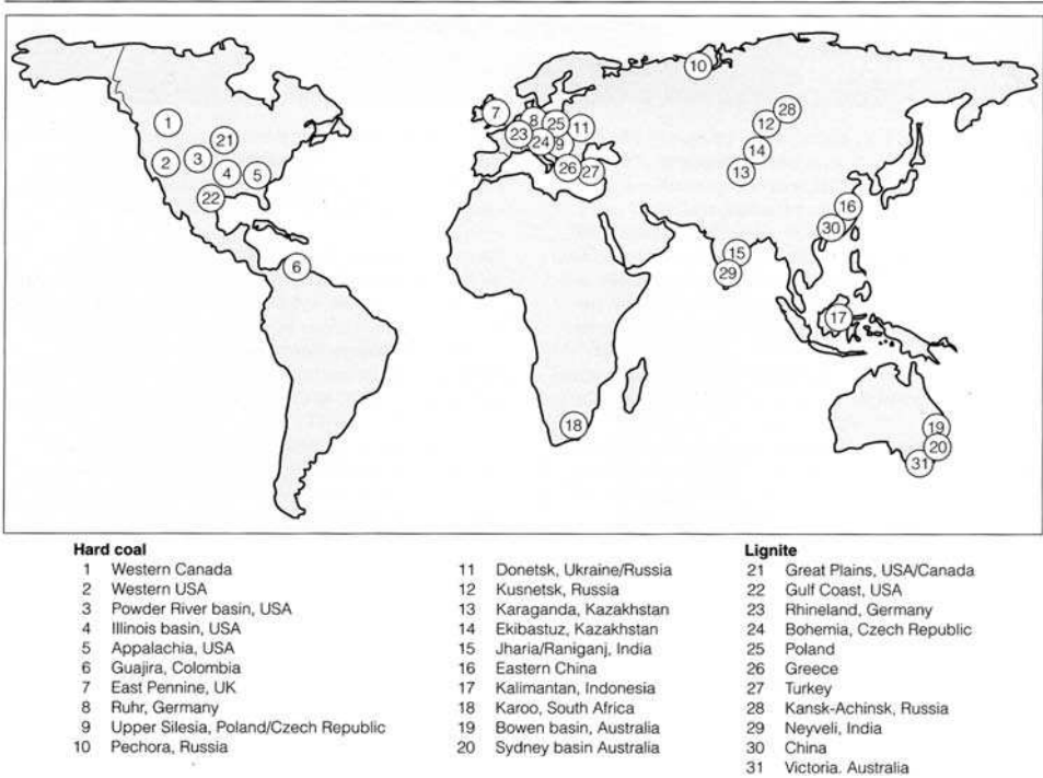
Figure 13.3 Location of the world's major hard coal (bituminous, anthracite) and lignite basins. (From Walker, S., 2000, Major Coalfields of the World: IEA Coal Research: The Clean Coal Centre, London , Fig. 1, p. 8, reproduced by permission.)
