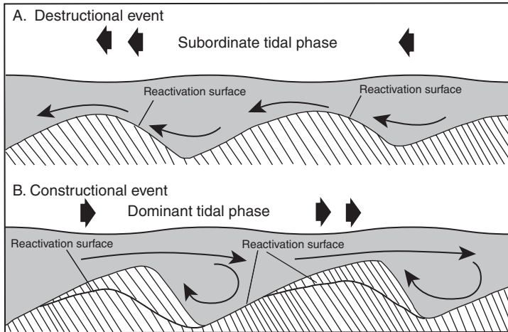
Figure 3.12 Schematic representation of reactivation surfaces in rippled sand caused by erosion of previously formed ripples during a subordinate tidal phase (destructural event) followed by renewed deposition during a dominant tidal phase (constructural event). (Based on Klein, 1970, Depositional and dispersal dynamics of intertidal sand bars: J. Sediment. Petrol. , 40 , Fig. 28, p. 1118.)
