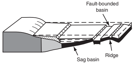
D. Basins floored by oceanic crust
