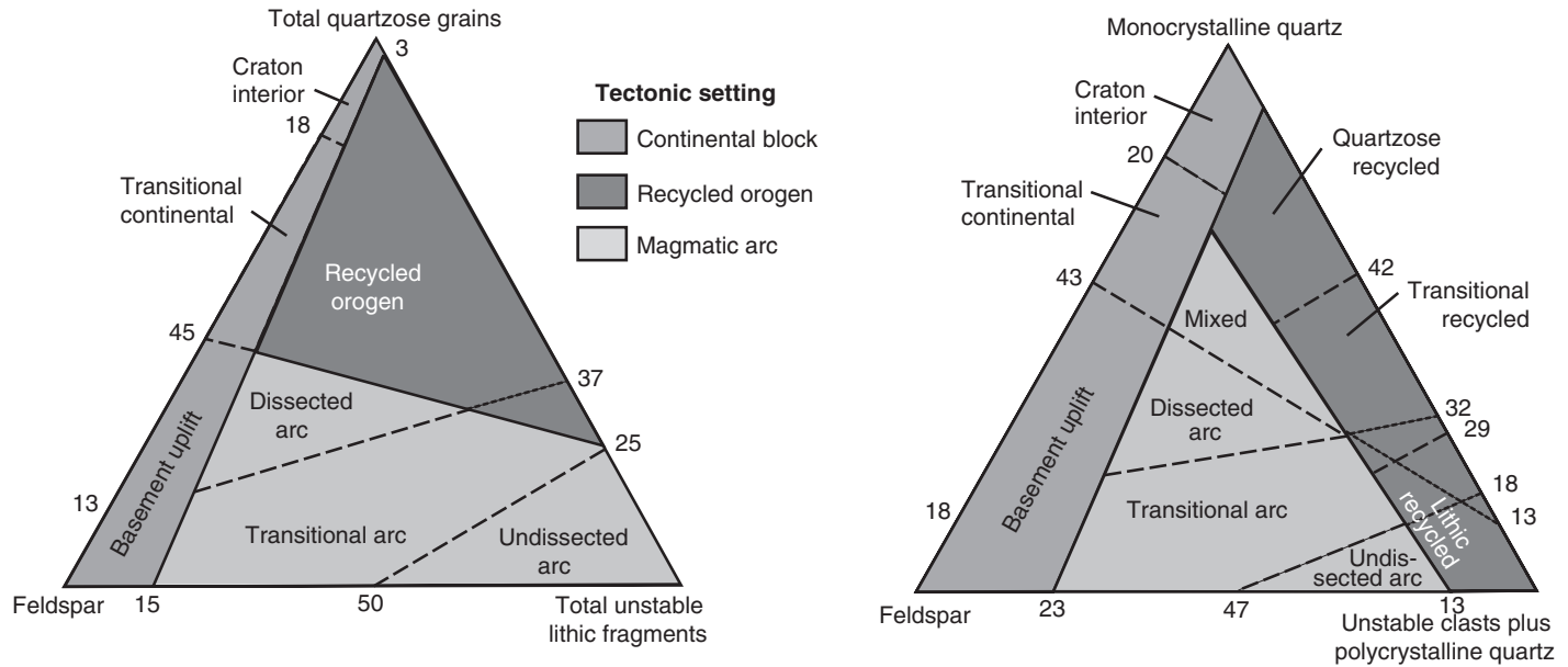
Figure 7.12 Relationship between framework composition of sandstones and tectonic setting, as indicated in Table 7.4. (After Dickinson, W. R. et al. , 1983, Provenance of North American sandstones in relation to tectonic setting: Geol. Soc. Am. Bull. , 94 , Fig. 1, p. 223.)
