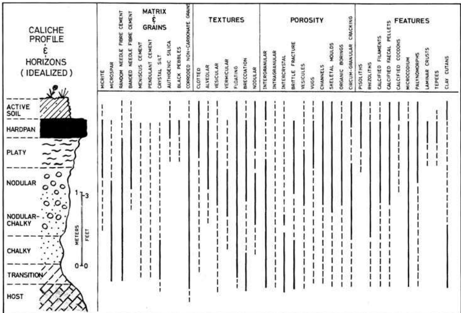
Figure 9.44 Idealized caliche profile and the distribution of major characteristics within the profile. [After Esteban, M. and C.F. Klappa, 1983, Subaerial exposure environment, in Scholle, P. A., D.G. Bebout, and C.H. Moore (eds.), Carbonate Depositional Environments : AAPG Memoir 33, Fig. 7, p. 5, reproduced by permission of AAPG, Tulsa, OK.]
