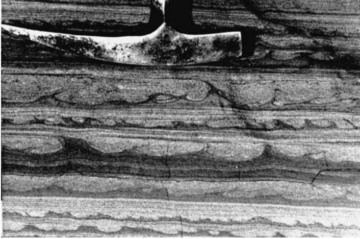
Figure 3.22 Multiple sets of small-scale flame structures in a thinly bedded and laminated siltstone–mudstone sequence. Elkton Siltstone (Eocene), southwestern Oregon. Note hammerhead for scale.
