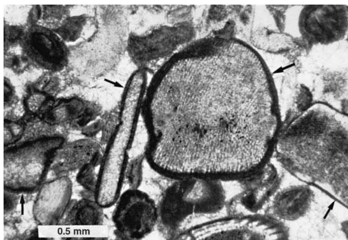
Figure 9.13 Micrite envelopes (arrows) developed around echinoderms and other fossil fragments. Renault Formation (Mississippian), Missouri. Crossed nicols.
