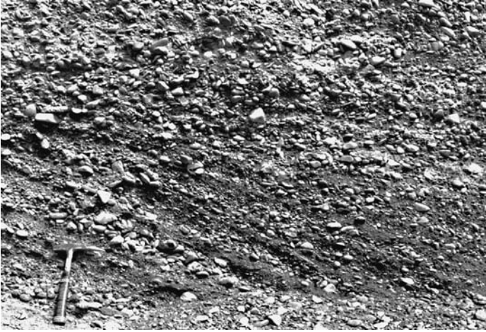
Figure 5.8 Stratification in Pleistocene beachface gravels, Cape Blanco, southern Oregon coast.
