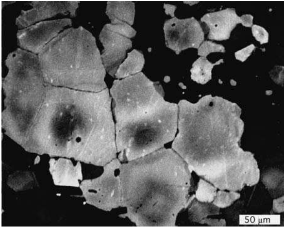
Figure 7.7 Cathodoluminescence image of metamorphic quartz showing mottled texture. Contact-metamorphosed hornfels, Japan. Specimen courtesy of Professor Hideo Kagami.
