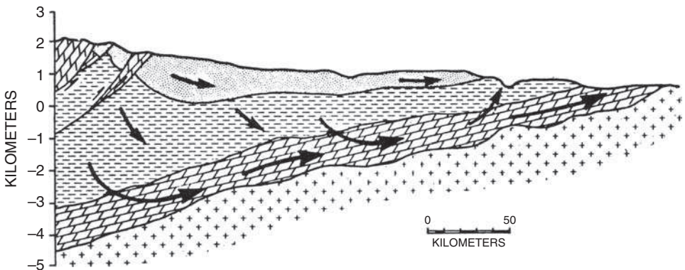
Figure 10.11 Conceptual model of topography-driven fluid flow in a sedimentary basin. Flow is driven by the hydraulic head of fluid resulting from meteoric recharge. The geometry of the flow system (arrows) is controlled by the water-table configuration and the permeability distribution in subsurface formations. (From Garvin, G. and R. A. Freeze, 1984, Theoretical analysis of the role of groundwater flow in the genesis of stratabound ore deposits: Am. J. Sci. , 284 , Fig. 3, p. 1091, reprinted by permission.)
