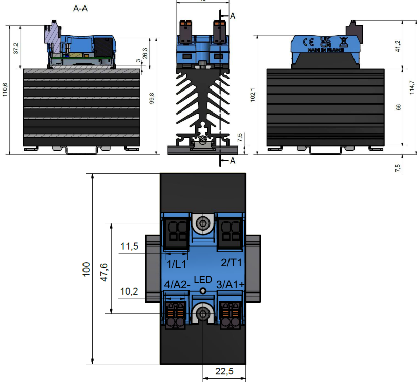
Dimensions (mm)
