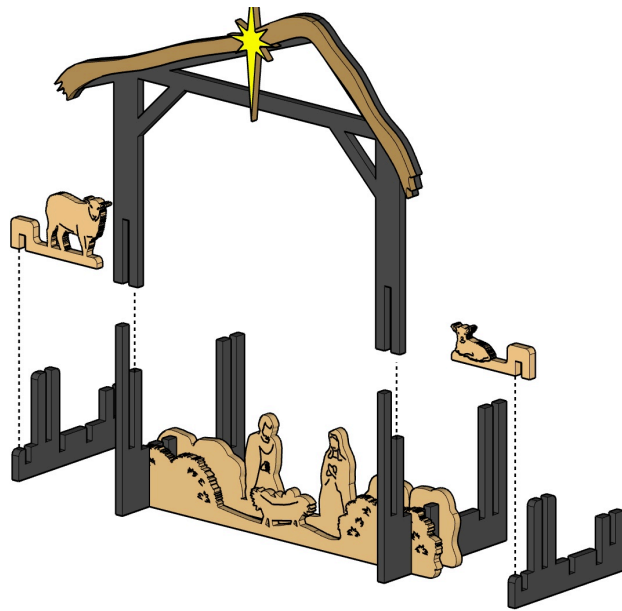
Step 5 - Add Front Wall and Sheep
