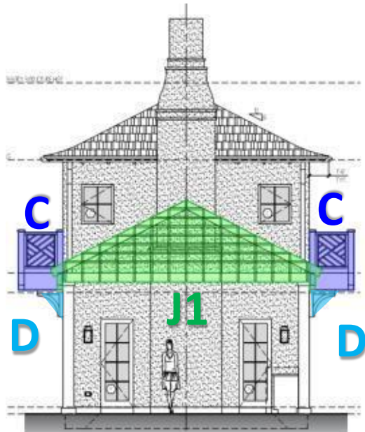
WEST ELEVATION - POOL HOUSE A 2.2
