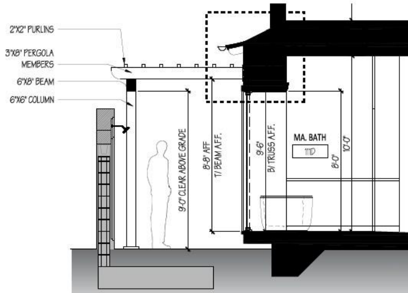
SECTION AT OUTDOOR SHOWER
