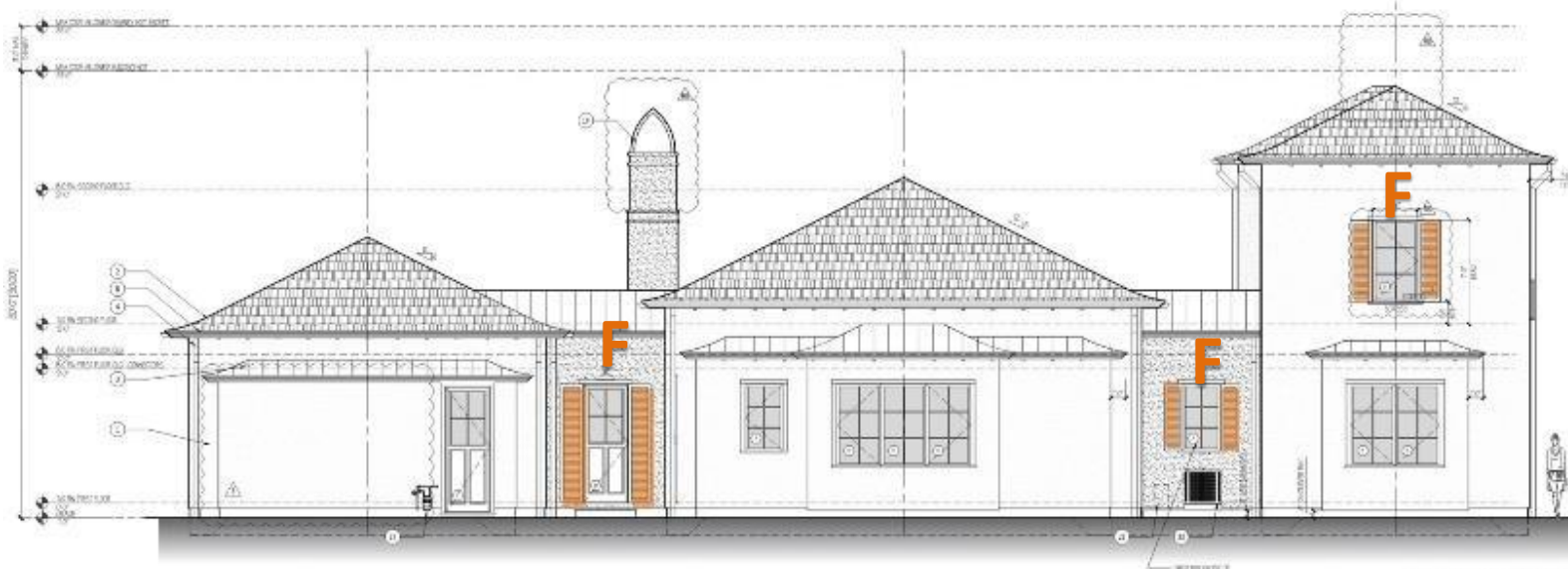
EAST ELEVATION - MAIN HOUSE A 2.2
