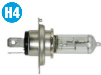
H4 26.006 H4 24V 75/70W - P43T-38 1900/1200LM - BRANCA
