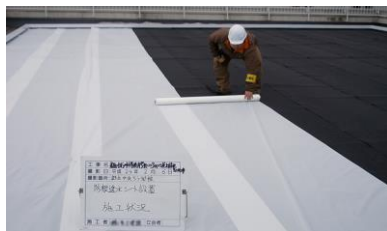
(5) Overlaying of a non-woven cloth root barrier
