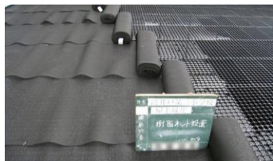
(4) Installation of industrial resin nets to prevent the charcoal bags from falling into the units
