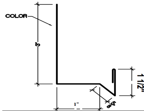
Special Jtrim W/Drip
