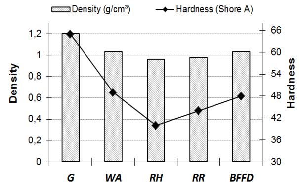
Figure 1. Density and hardness of carburized corncob ash filling compounds.
