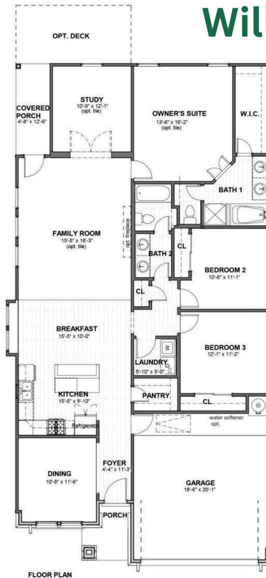
FLOOR PLAN
