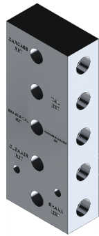
LYNX-1212 HYD,BLOCK,ALUM,ROW UNIT
