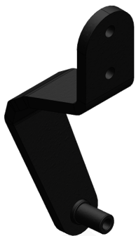
LYNX-0539 WLDT,CLOSER ARM,LF,ROW UNIT
