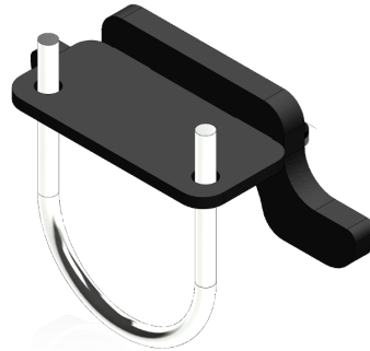
LYNX-1430 WLDT,SHANK STOP,ROW UNIT
