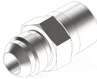
LYNX-1037 HYD,FTG,08MJ-08MP-0
