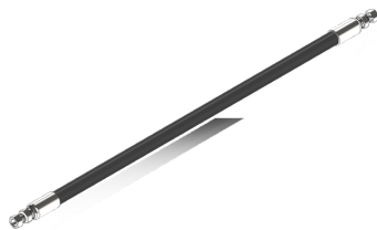
LYNX-1827 HYD,04-HOSE,06FJS0-06FJS0,19"
