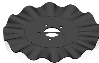
LYNX-1131 COULTER,4mm X 16" X 13 WAVE,5 ON 4 1/4",17/32" RD HOLE SIZE,2
