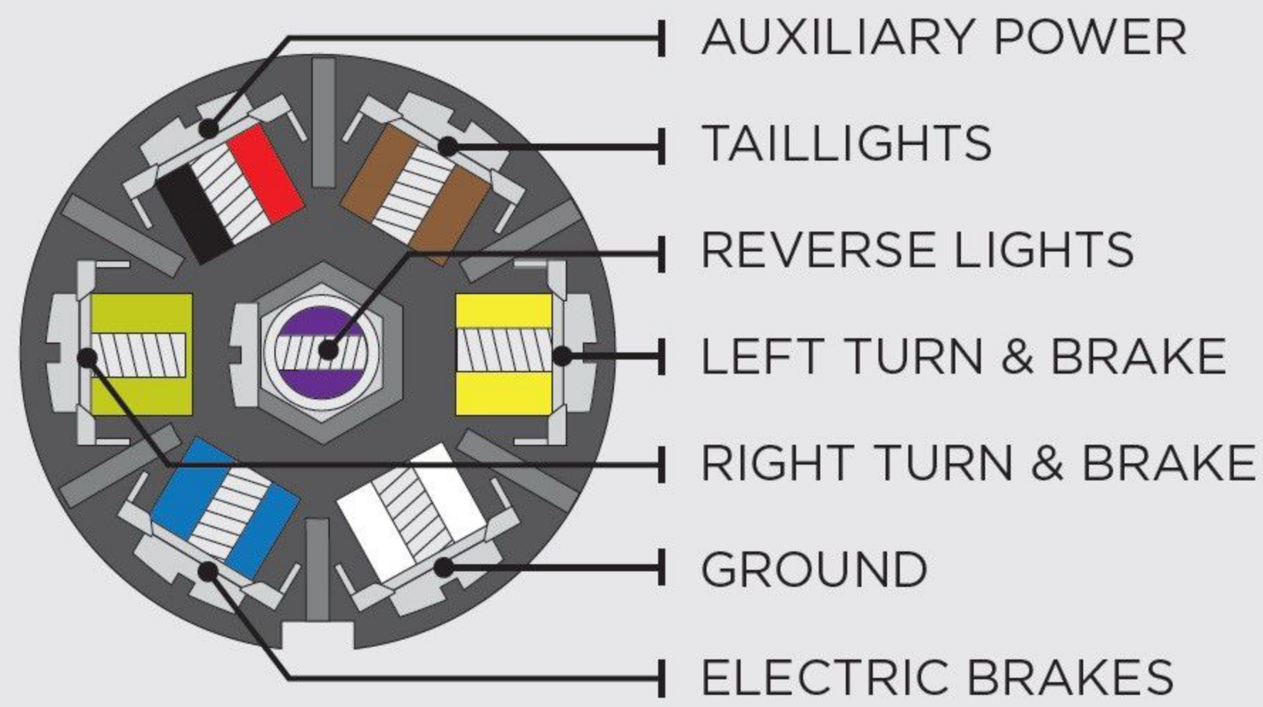
7 BLADE (SAE STANDARD)
