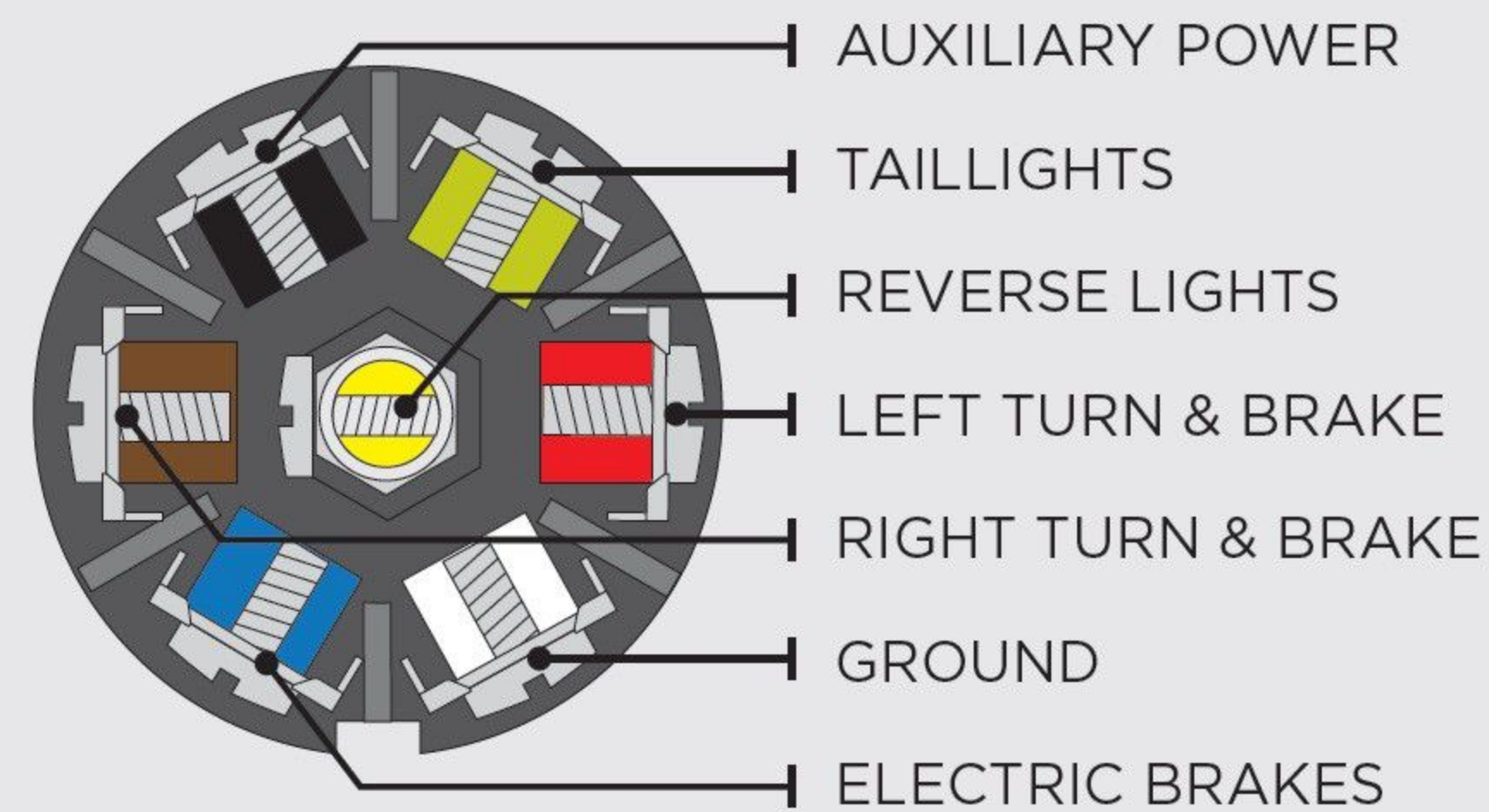
7 BLADE (RV STANDARD)
