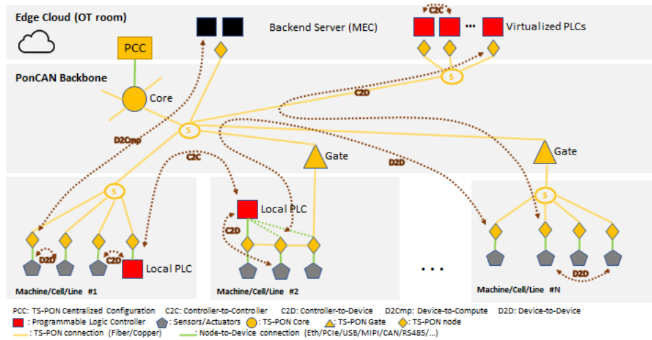
Figure 3 TS-PON factory automation application block diagram
