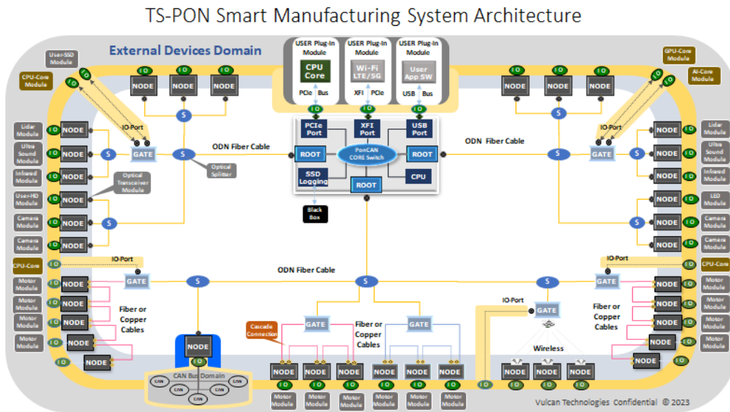
Figure 1 TS-PON network system architecture
