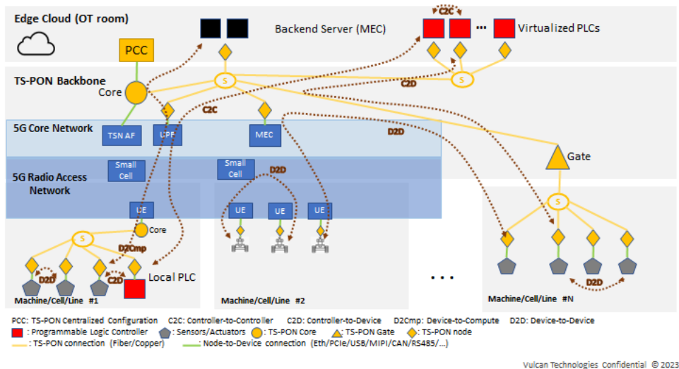
Figure 4 The integrated network of TS-PON and 5G
